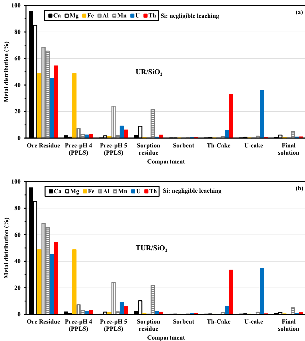
Fig. 9. Distribution of selected metals (or metalloids) along the extraction process summarized in Scheme 2 for UR/SiO 2 (a) and TUR/SiO 2 (b) sorbents (Si element being negligibly leached is not represented in the figure; the values of metal distribution are referred to total contents in the ore; reported data concern the experiments performed with the sorption step at pH 0 : 5).
