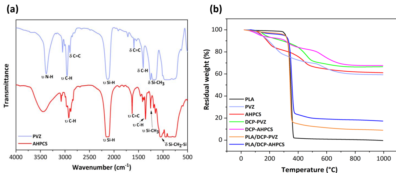
Figure 1. (a) FT-IR spectra of AHPCS and PVZ. (b) TGA plots recorded between room temperature and 1000 ^{\circ}\text{C} under inert atmosphere on PVZ and AHPCS, DCP-PVZ and DCP-AHPCS, PLA molds coated with preceramic polymers i.e., PLA/DCP-PVZ and PLA/DCP-AHPCS.
