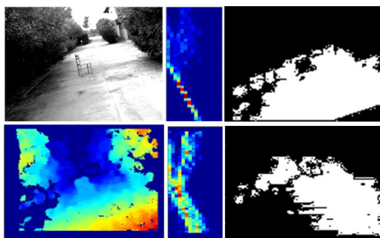
Figure 4: Upper left: Input greyscale image. Bottom left: disparity map. Upper right: raw output of the ground segmentation process with accelerometer. Bottom right: output of the ground segmentation process without accelerometer (white=ground). Corresponding V-Disparity images in the middle column.
