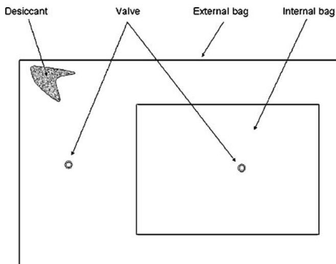
Fig. 1 Double-layer Tedlar bag with the possibility of incorporating desiccant inside
