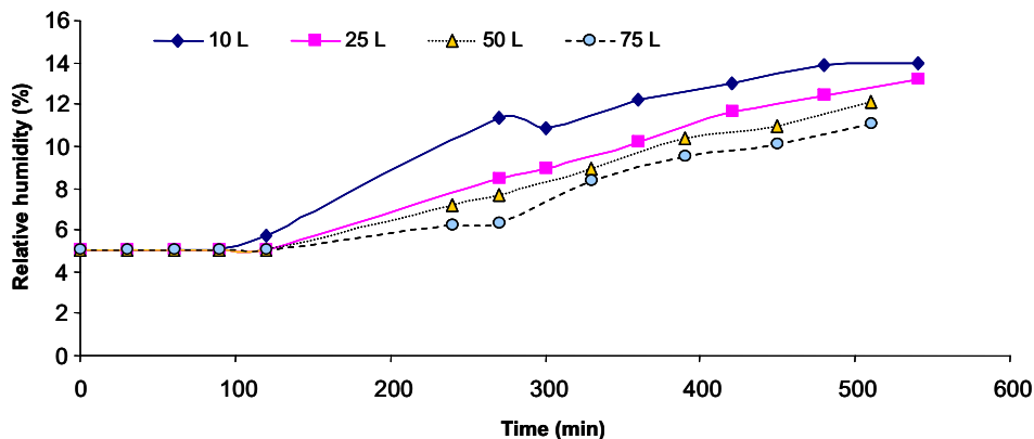
Fig. 6 Evolution of humidity in internal bags with different volumes of dry air in external bags
