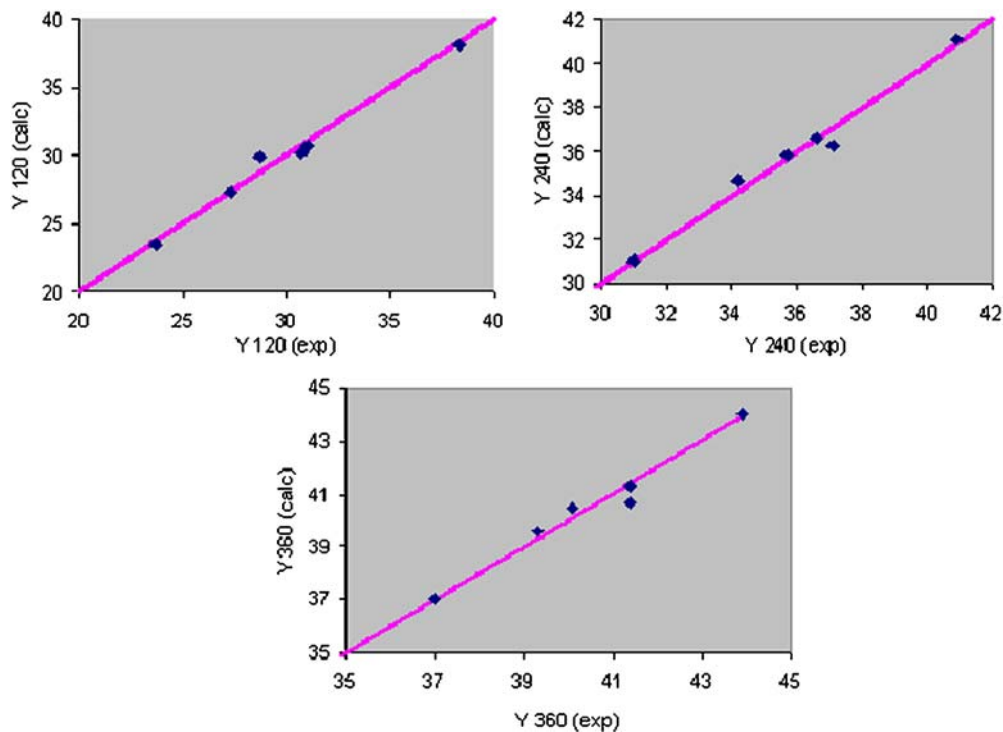
Fig. 5 Deviation between experimental data and calculated data with the three models
