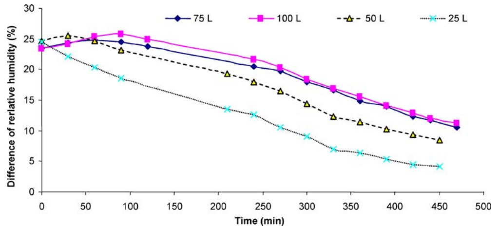
Fig. 3 Difference between internal humidity and room humidity in Tedlar bags with different volumes (initial relative humidity of the room was 25%)
