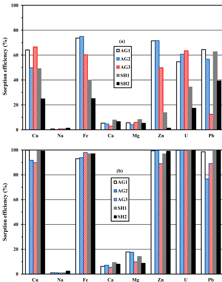
Fig. 6. Sorption efficiency for the treatment of water samples collected from Sinai wells after pH control at (a) pH_0 \approx 2 and (b) pH_0 \approx 5.5 (SD: 0.2 \text{ g L}^{-1} ; time: 5 h; T: 22 \pm 1 \text{ }^\circ\text{C} ; v: 210 rpm).
