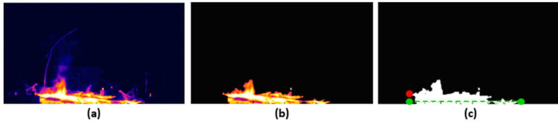
Fig. 19. Example of the results obtained from: (a) an original IR frame, (b) the segmented image and (c) the calculation of the corresponding fire width for test 3 at 621 s.
