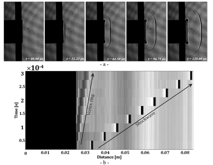
Fig. 3. a - Shadowgraphs of shock wave propagation and the vortex ring emergence. b - Grayscale intensity profile (streak image) on the aerodynamic axis representing the time propagation of the vortex ring and the shock wave.
