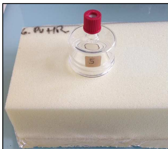
Figure 1. Pictures showing the emission cell placed on the material surface before sampling (a) and SVOCs sampling by SPME in the cell (b).
