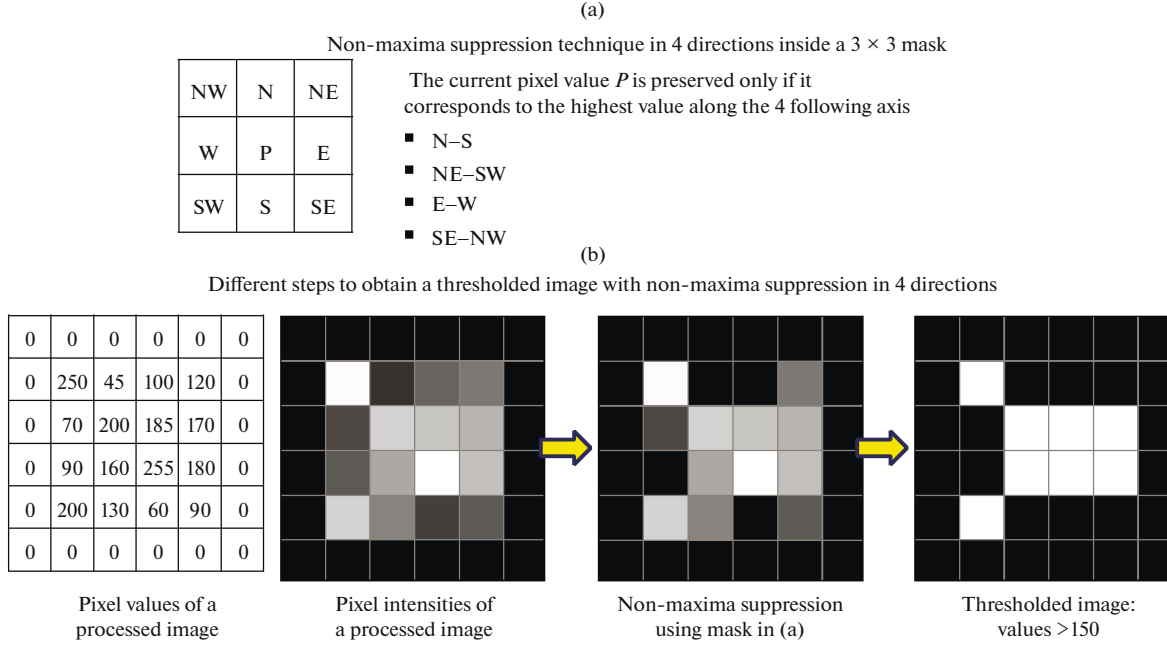
Fig. 5. Non-maxima suppression technique and different steps to obtain a thresholded image in 4 directions (usually used for ridge/valley detection with DOLD or Laplacian).
