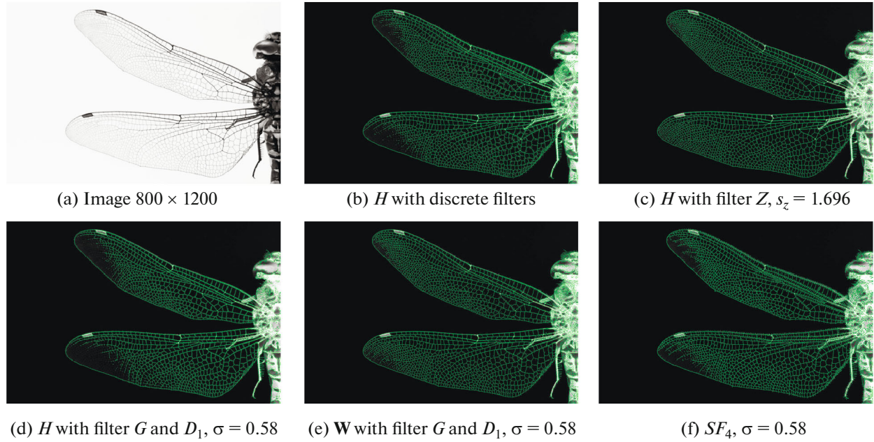
Fig. 16. Valley detection in green on real image of a dragonfly, with thin, blurred, and very close junctions. The original image is inverted for a better visualization.
