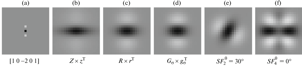
Fig. 11. Two-dimensional discrete filters for valley detection in y direction of width 7, parameters are available in Table 1. The negative of filters detect ridges.
