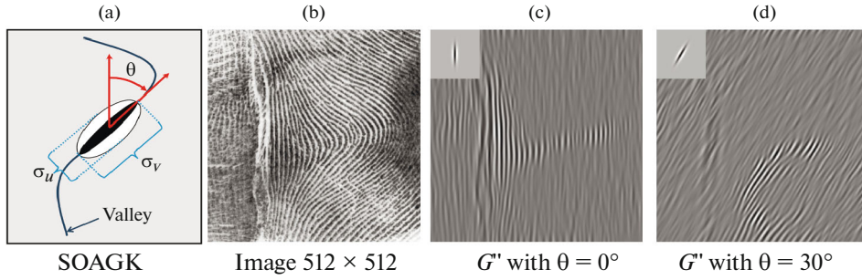
Fig. 12. Representation and visualization of the second derivative of an image computed by convolution with the SOAGK with \sigma_u = 2.88 and \sigma_v = 5\sigma_u .
