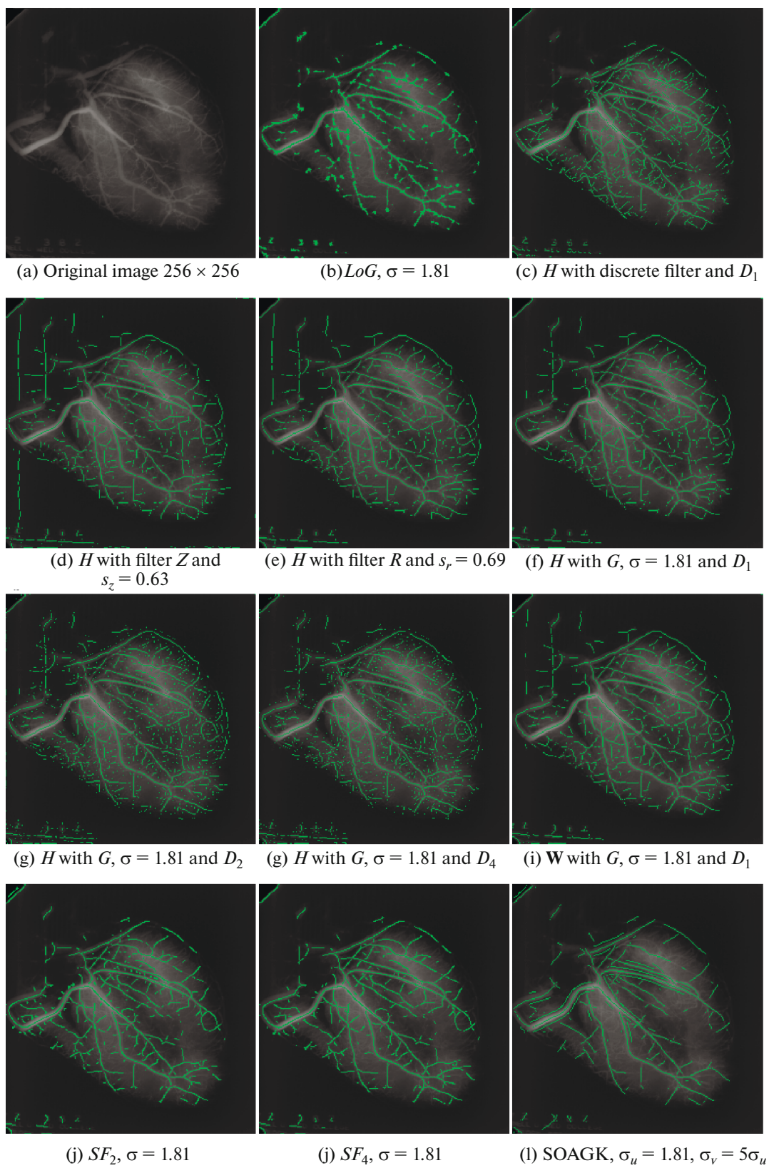
Fig. 21. Ridge detection on heart image. Detected ridges are displayed on the original image. Thresholded images correspond to the 3500 highest computed points for each method.
