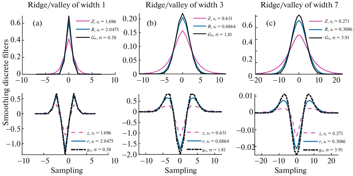
Fig. 10. Visual comparison of tested normalized 1D low-pass filters and 2nd order filters with the ideal parameters tied to the width of the ridge/valley.
