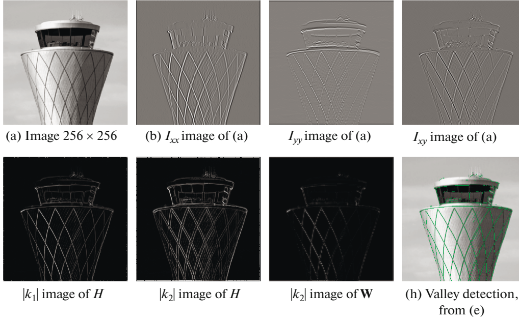
Fig. 6. Image derivatives and eigenvalue images using Hessian matrix (Eq. (3)) or Weingarten \mathbf{W} (Eq. (6)).
