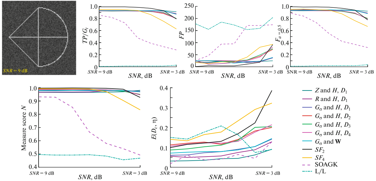
Fig. 17. Evaluation of the different ridge/valley extraction techniques on synthetic images corrupted by Poisson noise.
