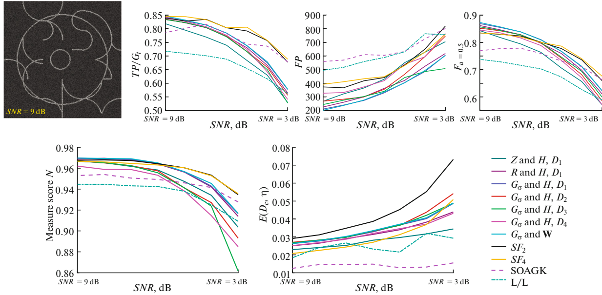
Fig. 18. Evaluation of the different ridge/valley extraction techniques on synthetic images corrupted by speckle noise.
