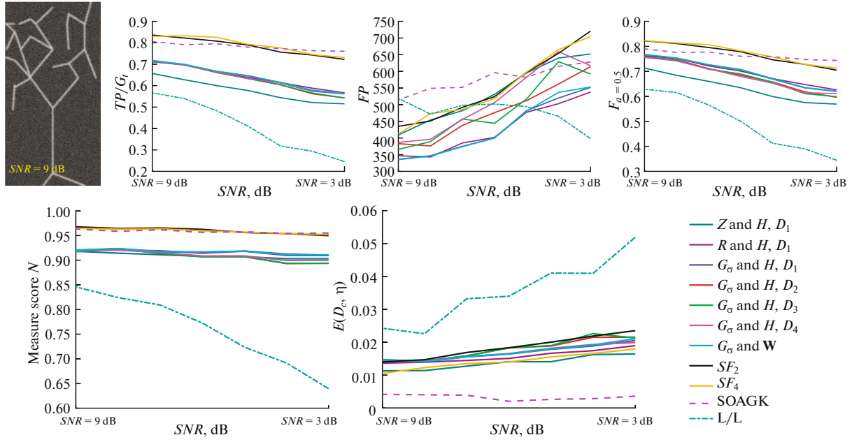
Fig. 19. Evaluation of the different ridge/valley extraction techniques on synthetic images corrupted by Gaussian noise and Gaussian blur.
