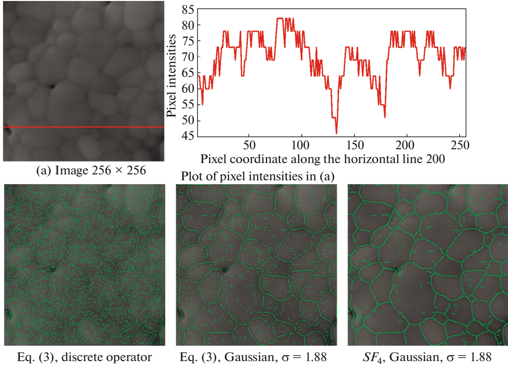
Fig. 7. Comparison of valley detection on real images. The image in (a) is obtained using scanning electron microscopy of melt ceramic. Here, the valleys are detected with 3 different techniques: Hessian matrix \mathcal{H} (c) without and (d) with Gaussian \mathbf{G}_\sigma , respectively and steerable filter of order 4 ( SF_4 ) in (e).
