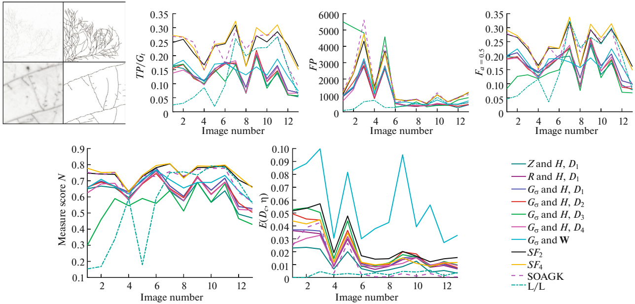
Fig. 20. Evaluation of the different ridge/valley extraction techniques on real images.
