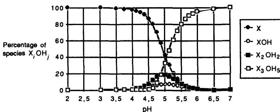
Fig. 3. Effect of pH on uranyl species repartition (10 ppm).
