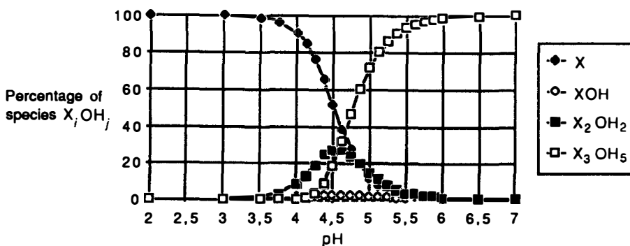
Fig. 4. Effect of pH on uranyl species repartition (100 ppm).
