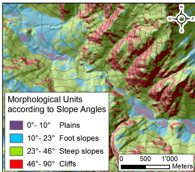
Fig. 4. Example of main morphological units in a region of the Bagnes valley according to slope angle thresholds got thanks to the SAD procedure. (Hillshade and 10 m isohypsies: ©2008 swisstopo).
