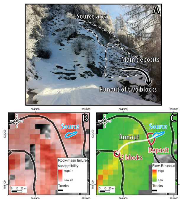
Fig. 10. (A) A recent rockfall event (2 January 2012) cut a mountain road with a deposit of approx. 1000 m 3 . The height difference between the fresh scarp and the road is about 30 m. (B) The rock-mass failure susceptibility map indicates that the onset is clearly defined as a potential rockfall source area with a high rock-mass failure susceptibility of about 0.8. (C) The trajectory of two blocks that reached a second road 80 m lower fit well with the predicted runout and confirms Flow-R results. (Hillshade: ©2008 swisstopo).
