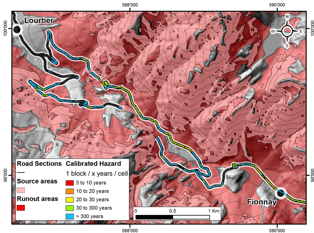
Fig. 9. Inverse hazard once the calibration has been performed, focused along the road section of Fionnay. Gaps along the section correspond to tunnels. (Hillshade and 10 m isohypsies: ©2008 swisstopo).
