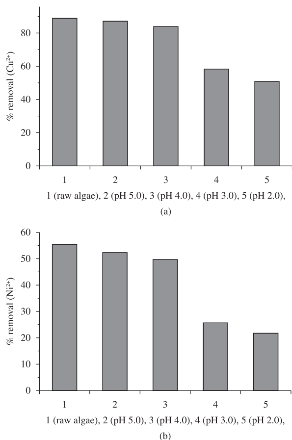
Figure 3. Comparison of a) \%\text{Cu}^{2+} removal; and b) \%\text{Ni}^{2+} removal of raw and acidified Sargassum filipendula .
