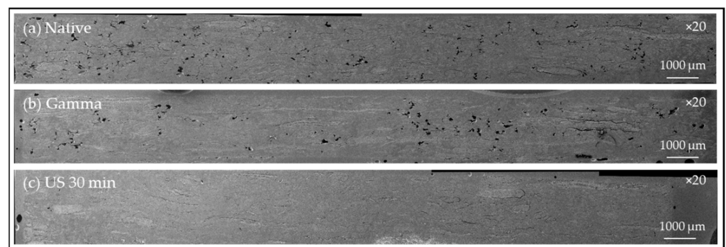
Figure 9. SEM observations of non-woven composites (a) Native; (b) Gamma; (c) US 30 min.
