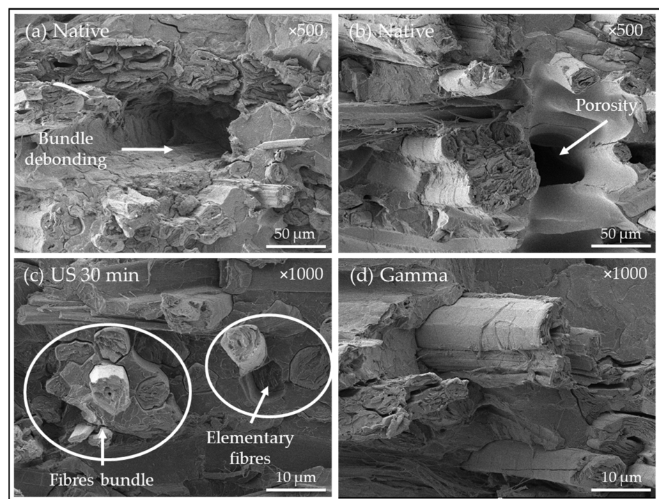
Figure 12. SEM observations of the interface of non-woven composites: (a) Debonding of fibre bundles; (b) porosity; (c,d) fibre bundles and elementary fibres in the US 30 min and Gamma composites, respectively.
