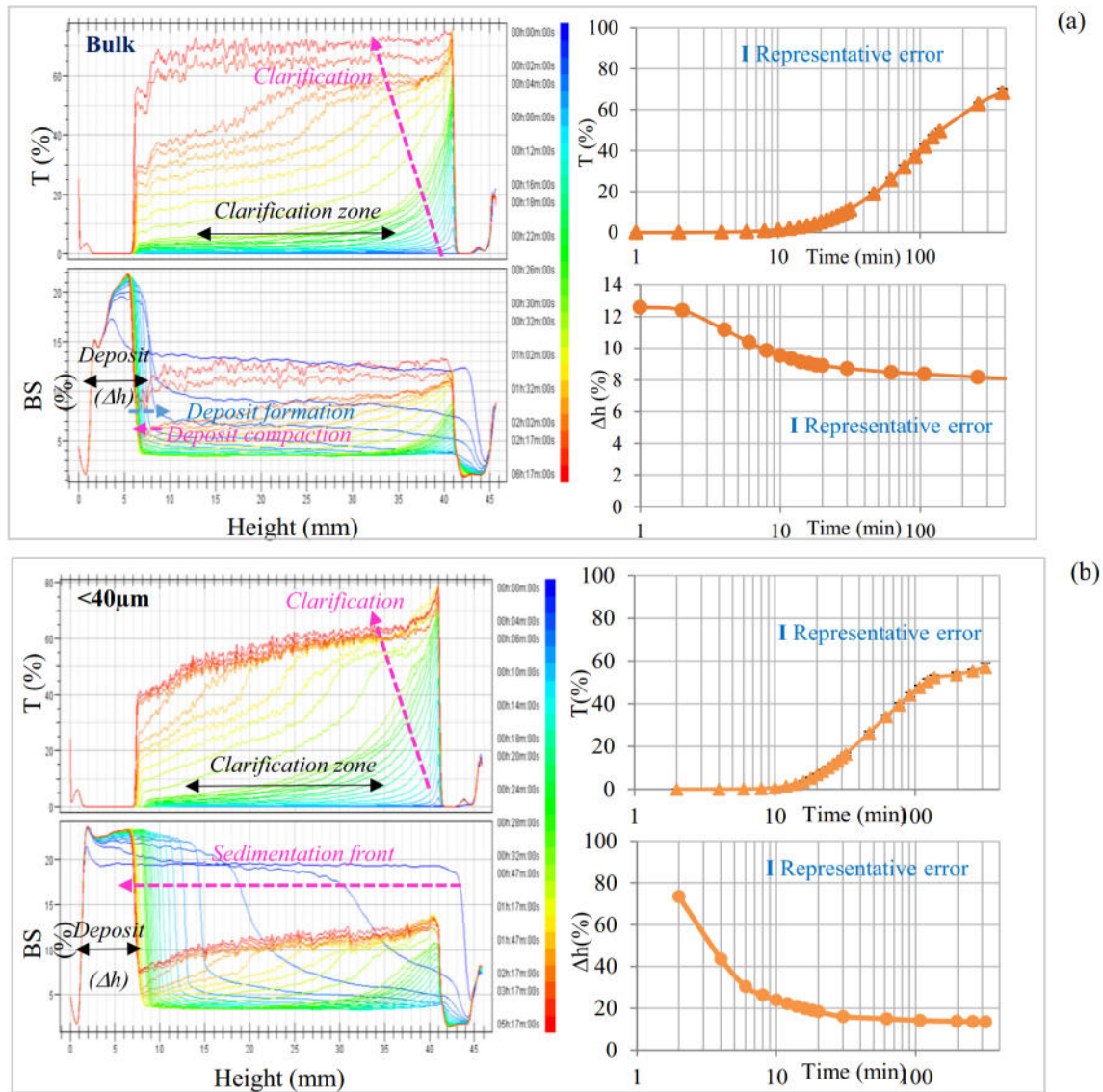
Fig. 7 Transmission profiles and the evolution of average transmission ( T ) over time and backscattering profiles and the deposit relative height evolution over time, during sedimentation process for the bulk fraction (a), and the fine fraction (b) of sediment from the channel
