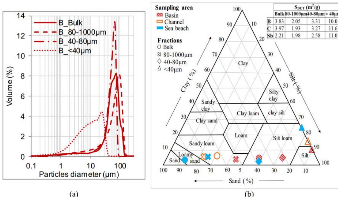
Fig. 3 Particle size distribution of bulk sediments ( < 1 \text{ mm} ) from the basin (a) measured in artificial seawater (A) and granular classification of the sediment in the USDA textural triangle and surface area (SBET) (b). Clay
