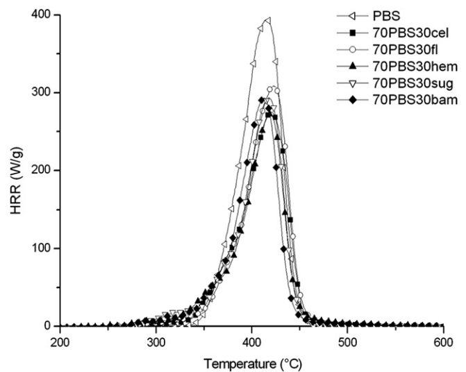
Fig. 5. PCFC curves of biocomposites based on various natural fibers.
