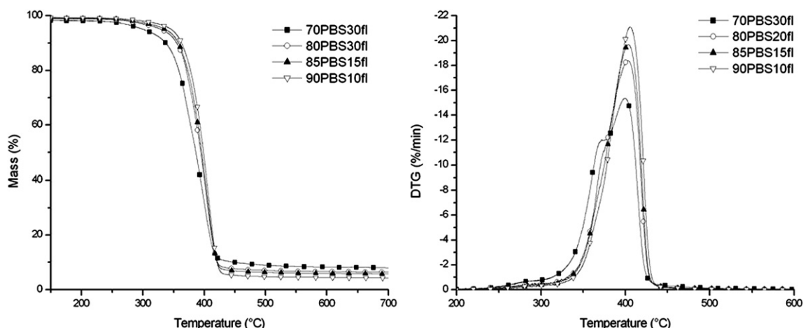
Fig. 9. TGA curves of various biocomposites comprising different amounts of flax fiber.
