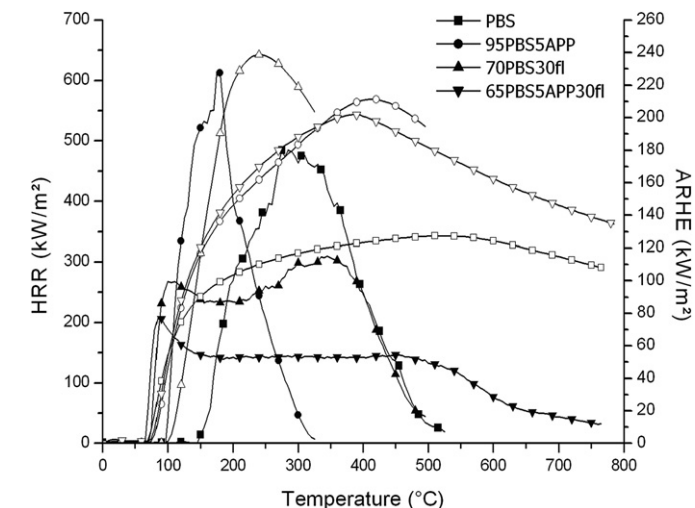
Fig. 13. Cone calorimeter curves of FR-biocomposites: the curves with full symbols represent the HRR vs temperature whereas the curves with empty symbols represent the ARHE vs temperature.
