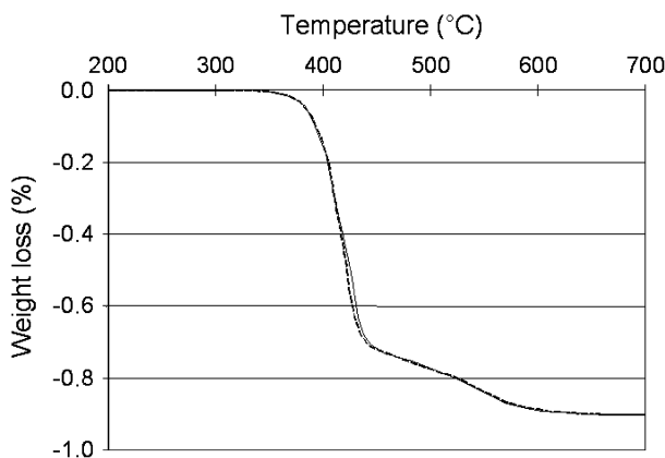
Figure 13. TGA curves (5°C/min) of PET filled with 3% red P + 2% \text{Fe}_2\text{O}_3 in air and argon. (—) in air, (---) in argon.
