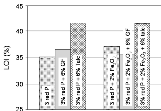
Figure 19. Limiting oxygen index (LOI) of PET compositions containing red P, Fe 2 O 3 , glass fibers (GF) or talc.
