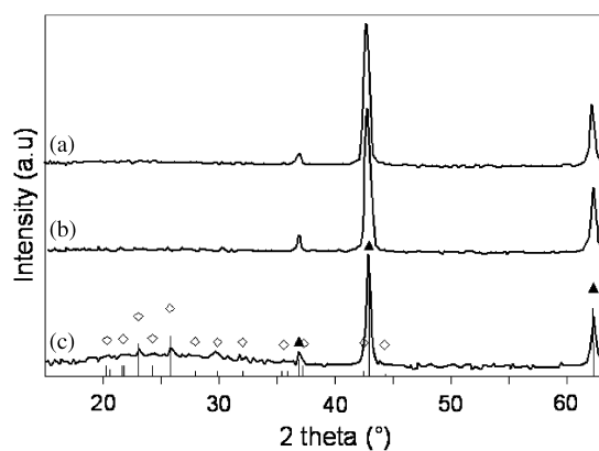
Figure 10. X-ray spectra of: (a) PET + 5% MgO; (b) MgO; and (c) PET + 3% red P + 2% MgO. As reference, diffraction patterns of MgO (▲) and \text{Mg}_3(\text{PO}_4)_2 (◇) are represented.
