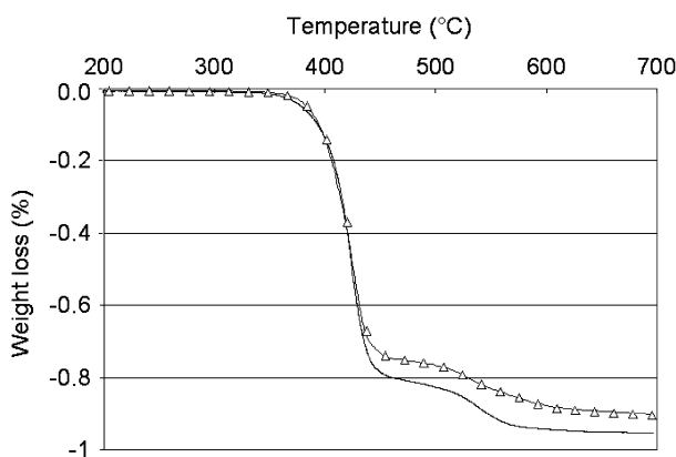
Figure 14. TGA curves in air (5°C/min) of filled PET. (Δ) 4% red P + 1% \text{Fe}_2\text{O}_3 , (—) 2% red P + 3% \text{Fe}_2\text{O}_3 .
