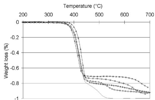
Fig. 2. TGA curves of filled and unfilled PET in air and argon (5 °C/min). (—) PET in air, (Δ) PET in Argon, (□) 3% red P, (*) 5% red P, (○) 3% red P + 2% Al 2 O 3 .
