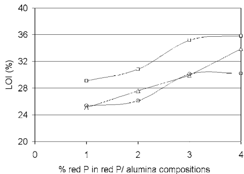
Fig. 7. Influence of the median diameter and specific surface area of alumina on the Limiting Oxygen Index of filled PET for several red P/alumina compositions. (△) red P, alumina (ATH calcinated at 700 °C) median diameter 2.5 \mu\text{m} , sBET = 130 \text{m}^2/\text{g} , synthetic alumina median diameter 0.5 \mu\text{m} , sBET = 5.6 \text{m}^2/\text{g} .
