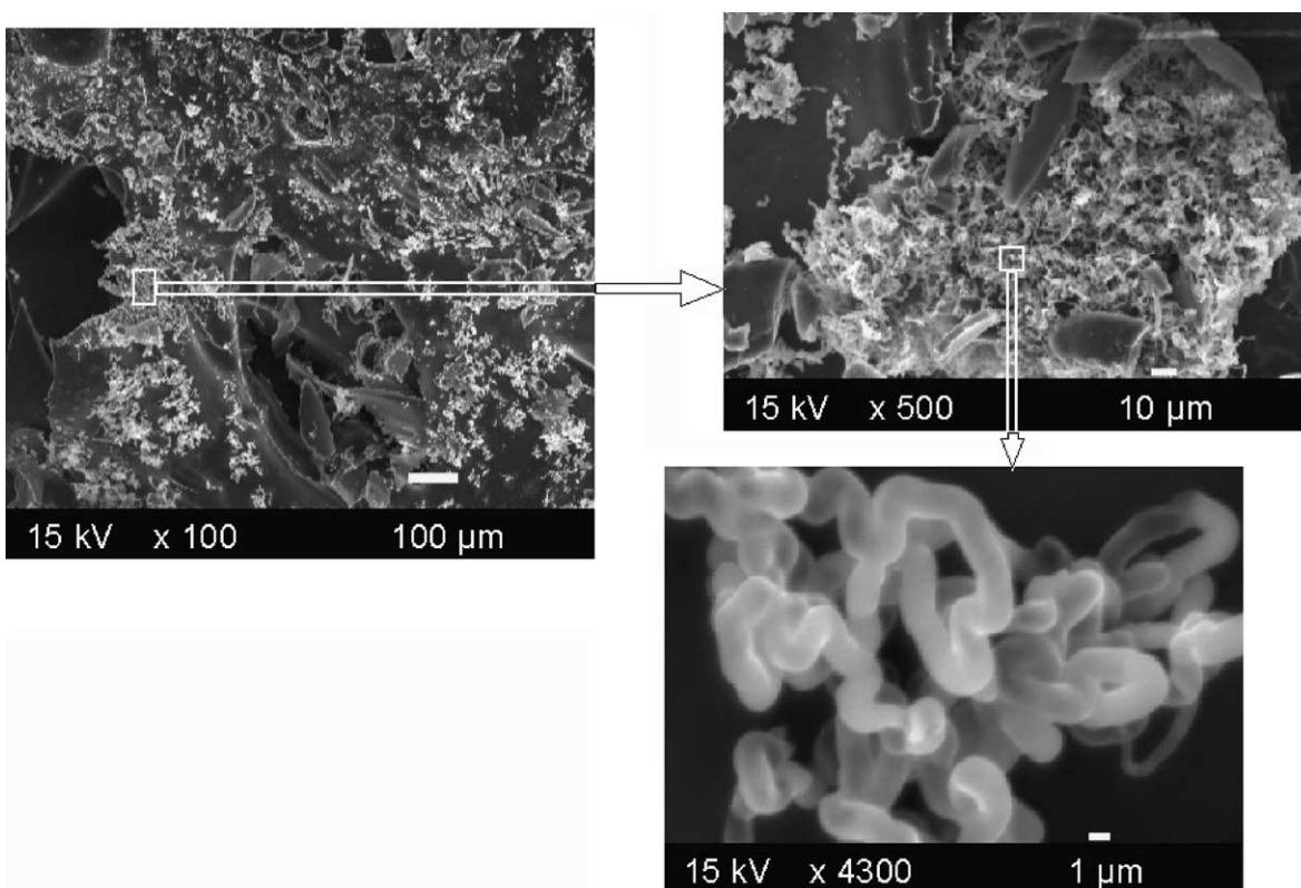
Fig. 11. SEM micrographs (×100, 500 and 4300) of the residue of (c) composition.
