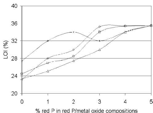
Fig. 6. Limiting oxygen index (LOI) of PET as a function of the red P/metal oxide composition. (□) red P/ \text{Al}_2\text{O}_3 , (○) red P/ \text{MgO} , (*) red P/ \text{Fe}_2\text{O}_3 , (△) red P.
