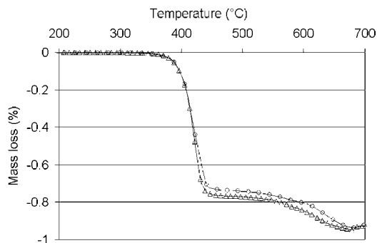
Fig. 8. TGA curves in air (5 °C/mn) of PET filled with 3% red P + 2% Alumina in function of the specific surface area of alumina, (○) \text{Al}_2\text{O}_3 sBET = 250 \text{m}^2/\text{g} , (△) \text{Al}_2\text{O}_3 sBET = 130 \text{m}^2/\text{g} .
