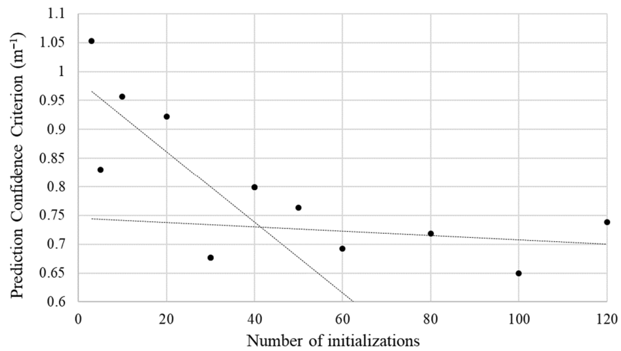
Figure 5. C_{PC} cross-validation score of ensemble models as a function of the number of members ( X ).
