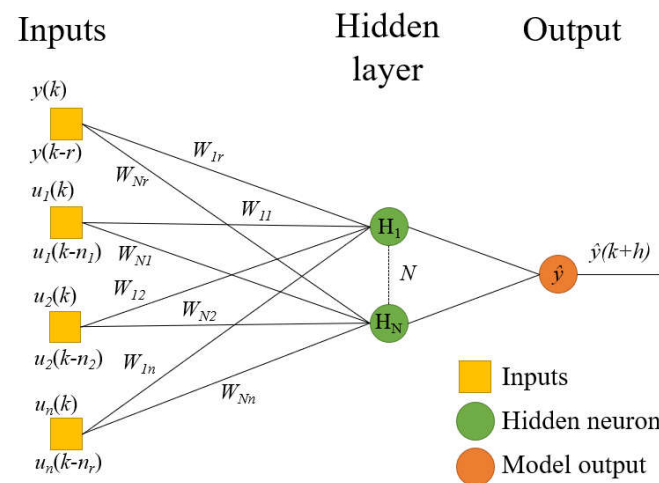
Figure 1. Multilayer Perceptron representation, with x_i , the exogenous variables; W , the matrix of parameters; y , the measured output; \hat{y} , the predicted output; r , the order of the model, n_r , the input window width; H_i ( i = 1 to N ) the hidden neurons; N , the number of hidden neurons; k , the discrete time and h , the lead time [13].
