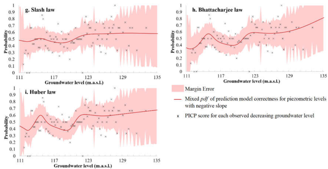
Figure 11. Models of correctness and Error margin ( M_E ), calculated from composite pdf of decreasing levels and using a confidence index of 95% for (a) Normal law, (b) Gumbel law, (c) Laplace law, (d) Raised Cosine law, (e) Cauchy law, (f) Logistic law, (g) Slash law, (h) Bhattacharjee law and (i) Huber law.
