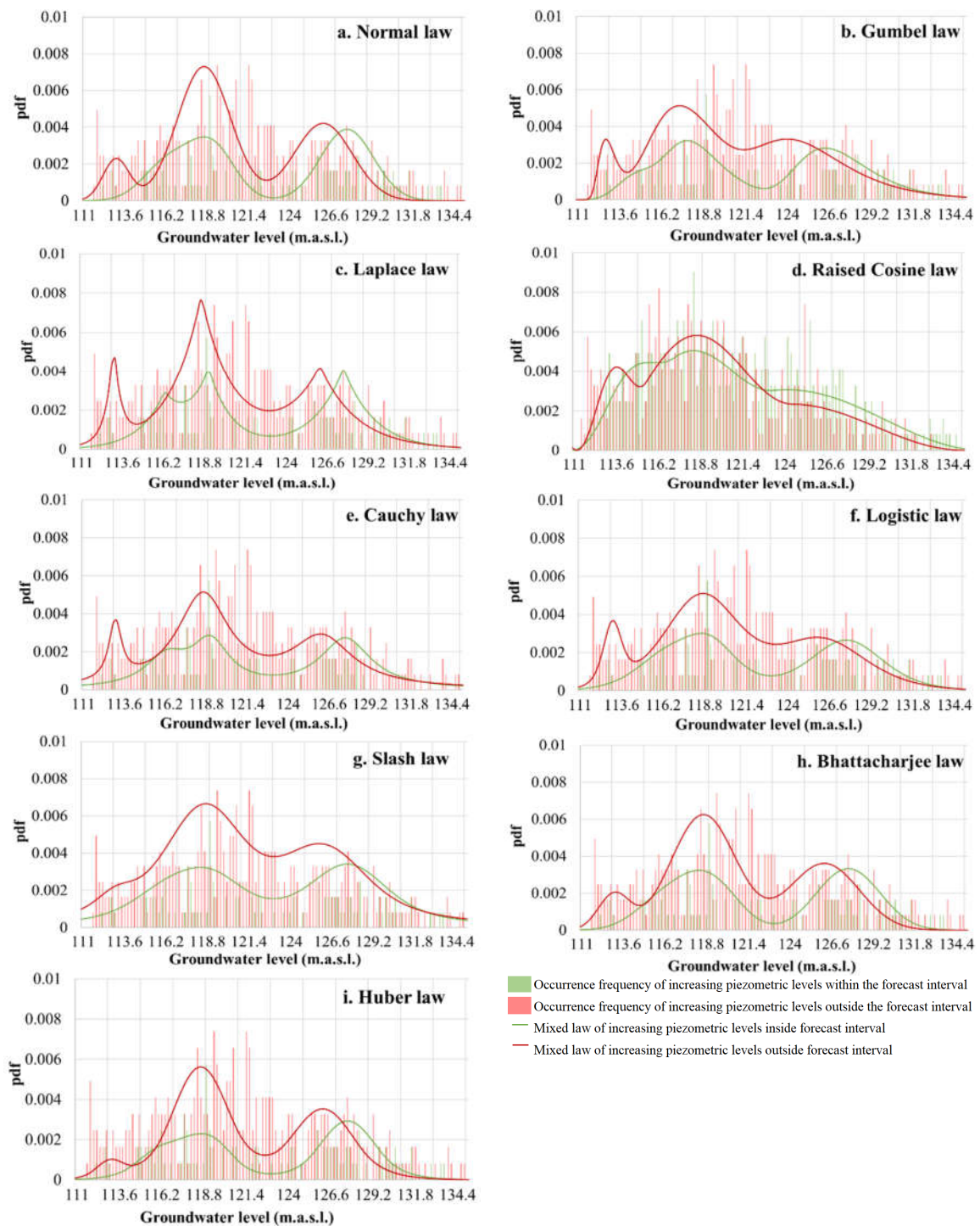
Figure 9. Mixed pdf for increasing groundwater distributions. with (a) Normal law, (b) Gumbel law, (c) Laplace law, (d) Raised Cosine law, (e) Cauchy law, (f) Logistic law, (g) Slash law, (h) Bhattacharjee law and (i) Huber law.
