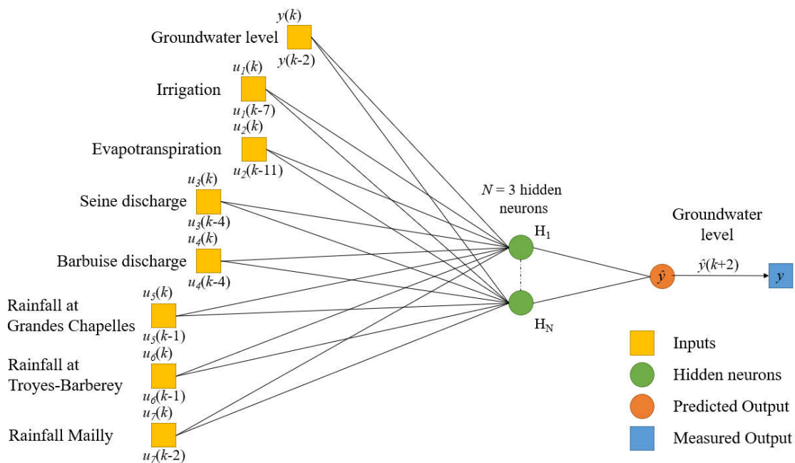
Figure 4. Selected architecture.
