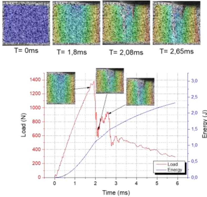
Figure 5 : TRDIC results of damage history growth, 83kfps. Color shows vertical deformation (light blue<0<red, white NAN)
