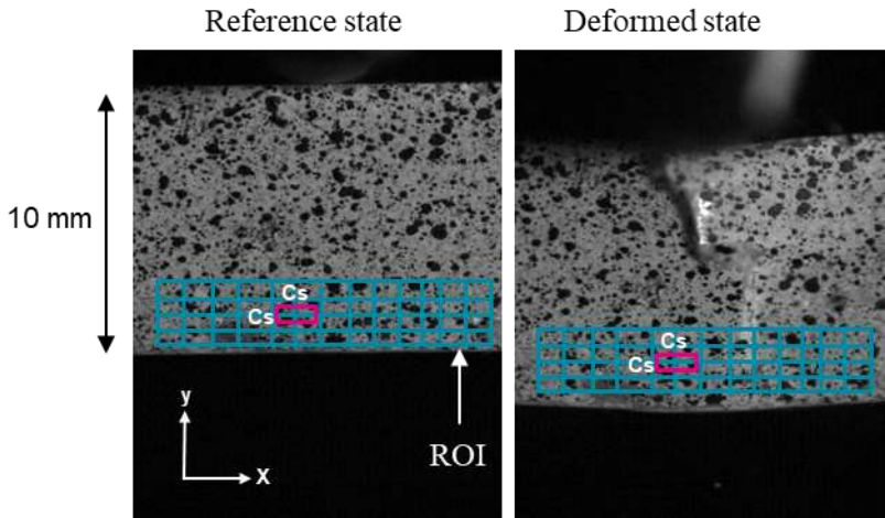
Figure 4 : Principle of image correlation with reference and deformed image
