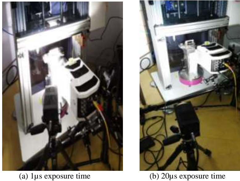
Figure 3 : Sample illumination at constant image intensity and contrast: (a) 1μs, (b) 20μs exposure time
