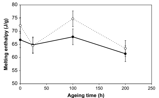
Fig. 13. Evolution of the melting enthalpy with ageing time for PA-6,6 composites reinforced by (●) ST PA66 glass fibres and (○) SP PA66 glass fibres.
