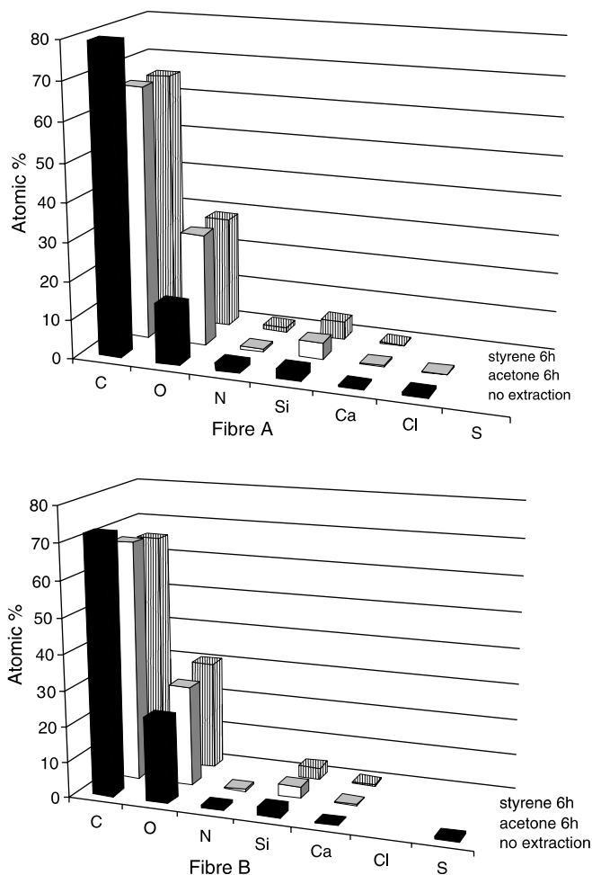
Fig. 4. Atomic % versus extraction for fibres A and B (● before extraction, ○ acetone 6 h, ● styrene 6 h).
