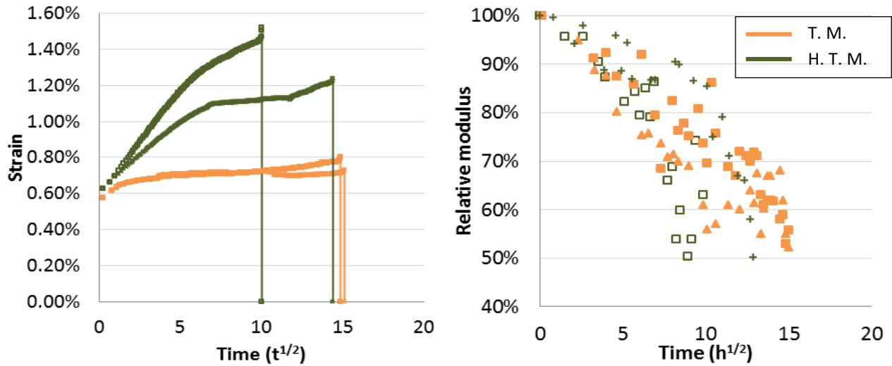
Figure 2 – Strain in function of ageing time for flax fibre composites exposed to thermos-mechanical and hydro-thermo mechanical degradation (at 50°C and 60 MPa).
