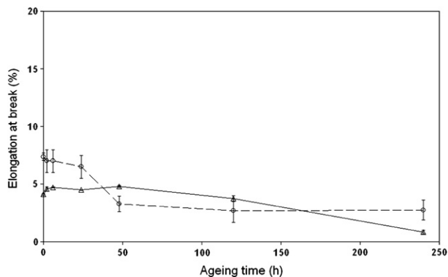
Fig. 3. Elongation at break of P(L)LA U and P(L)LA NW as a function of hydrothermal ageing (○) neat P(L)LA NW ; (△) P(L)LA U .
