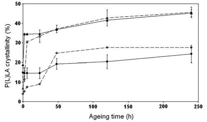
Fig. 8. Effect of blending with P \epsilon CL on P(L)LA NW and P(L)LA U crystallinity as a function of hygrothermal ageing (Δ) P(L)LA U ; (▲) P(L)LA U /P \epsilon CL; (○) P(L)LA NW ; (●) P(L)LA NW /P \epsilon CL.
