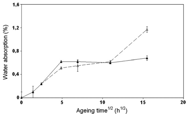
Fig. 7. Effect of blending with P \epsilon CL on P(L)LA U based blend water absorption as a function of hygrothermal ageing (Δ) P(L)LA U ; (▲) P(L)LA U /P \epsilon CL.
