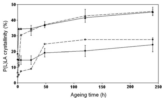
Fig. 8. Effect of blending with P \epsilon CL on P(L)LA NW and P(L)LA U crystallinity as a function of hygrothermal ageing (Δ) P(L)LA U ; (▲) P(L)LA U /P \epsilon CL; (○) P(L)LA NW ; (●) P(L)LA NW /P \epsilon CL.
