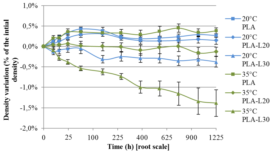
Figure 6 – Density variation in flax/PLA composites (ISO 1BA injected samples) depending on immersion time in water and temperature
