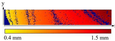
Figure 19: Reconstruction of the real sample thickness with method 5.2.
