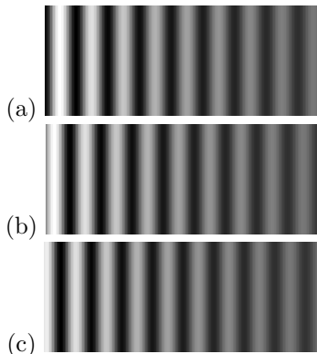
Figure 12: Noiseless far-infrared reflection images of the modelled sample at 279 GHz (a), 284 GHz (b) and 289 GHz (c). The grey-scale values corresponds to the measurement profiles in Fig.13.
