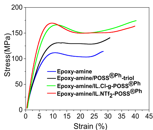
Fig. 5. Stress-strain curves of the neat epoxy-amine and the hybrid O/I epoxy networks.
