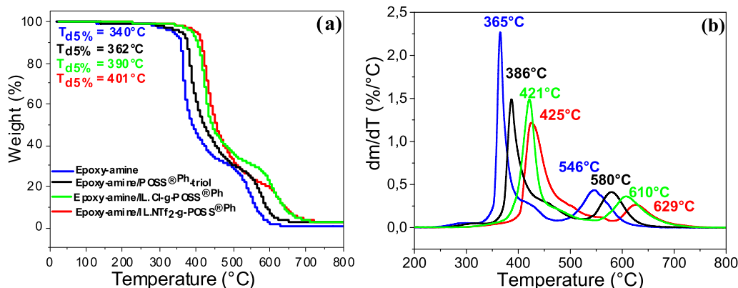
Fig. 6. a) Weight loss (TGA) and b) derivative of TGA curves (DTG) as a function of temperature for the neat epoxy-amine and the hybrid O/I epoxy networks under air atmosphere ( 10\text{ }^{\circ}\text{C min}^{-1} ).
