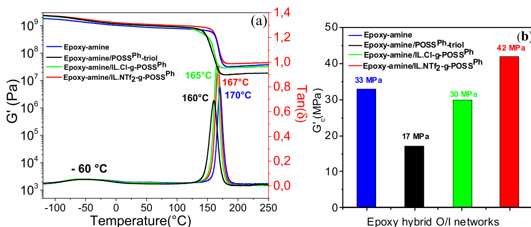
Fig. 4. a) Dynamic mechanical spectra and b) the shear storage moduli, G'_c (at 200 °C) of the epoxy-amine and the hybrid O/I epoxy networks containing POSS ® -triol and IL-g-POSS ® Ph with different anions (Cl - and NTf 2 ) at 1 Hz.
