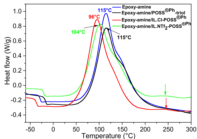
Fig. 1. DSC traces of neat epoxy-amine and the hybrid O/I epoxy reactive systems containing 5 wt % POSS Ph -triol or IL-g-POSS Ph with Cl - or NTf 2 anion (heating rate: 10\text{ }^{\circ}\text{C min}^{-1} ).
