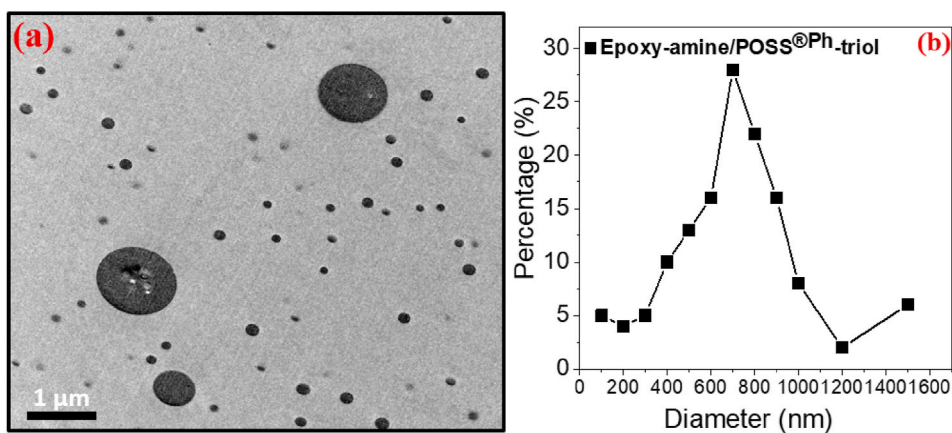
Fig. 2. a) TEM micrograph of the hybrid O/I epoxy network containing POSS Ph -triol, b) Size distribution of POSS Ph -triol aggregates.
