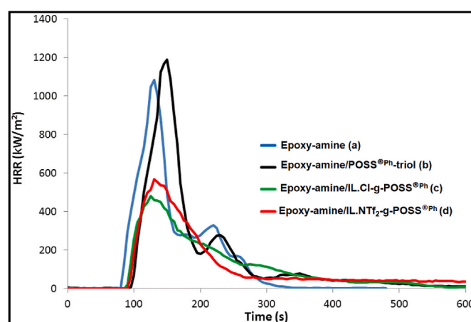
Fig. 8. Cone calorimeter HRR curves of the neat epoxy-amine, and the hybrid O/I epoxy networks.
