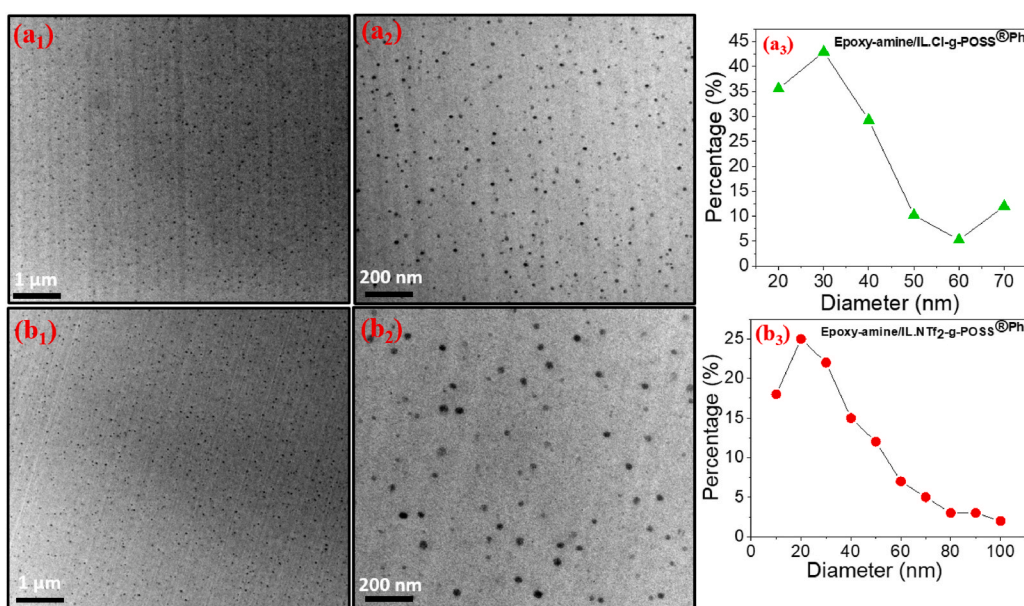
Fig. 3. TEM micrographs of the hybrid O/I epoxy networks containing: a) IL.Cl-g-POSS Ph at different magnification (a 1 ; a 2 ), b) IL.NTf 2 -g-POSS Ph at different magnification (b 1 ; b 2 ) and their size distribution (a 3 , b 3 ).
