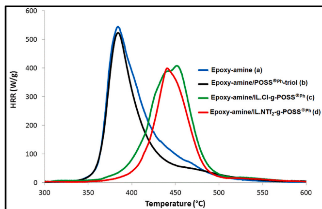
Fig. 7. PCFC HRR traces of the neat epoxy-amine, and the hybrid O/I epoxy networks.
