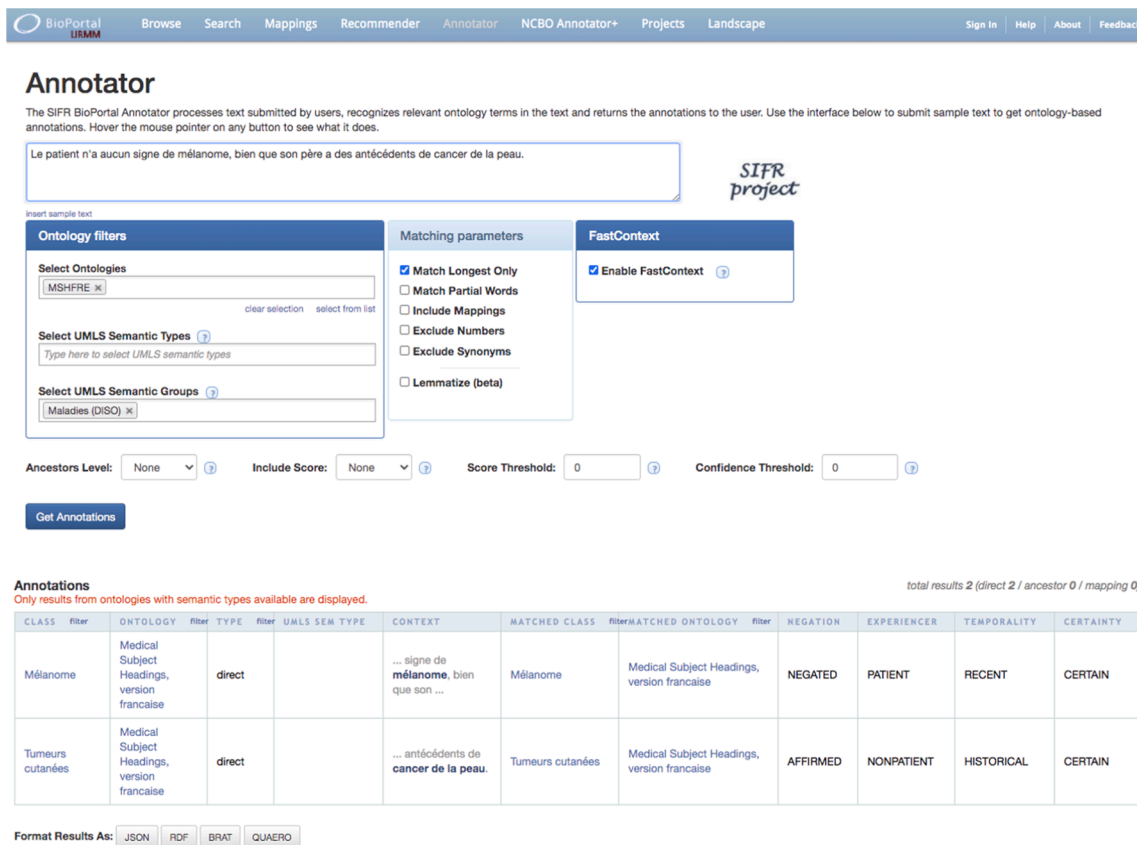
Fig. 1. SIFR Annotator user interface integrating the new contextual features. In this example, the target terminology is the French version of the Medical Subject Headings (MSHFRE) and the annotations are filtered to the ‘Disorders’ semantic group [29]. The semantic expansion (hierarchy and mapping) is not activated and only longest matches are kept.
