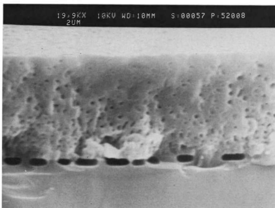
Fig. 10. Porous texture of \alpha\text{-alumina} from 1200°C to 1300°C.
