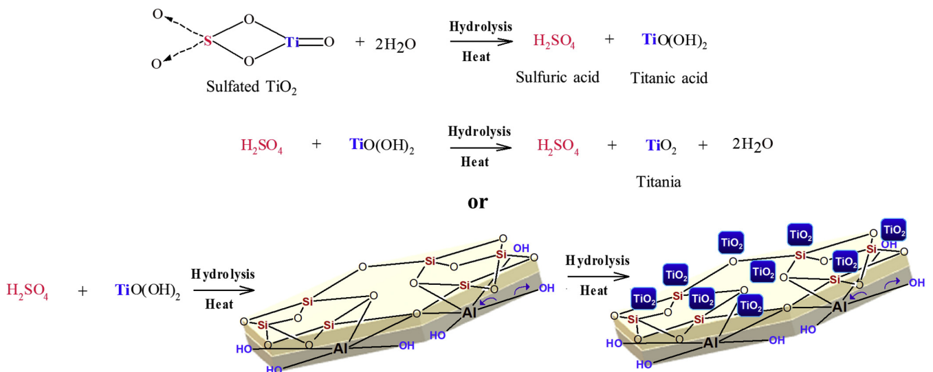
Fig. 10. Proposed mechanism for the adhesion of titania into the kaolinite based on sulfated \text{TiO}_2 sol-gel.
