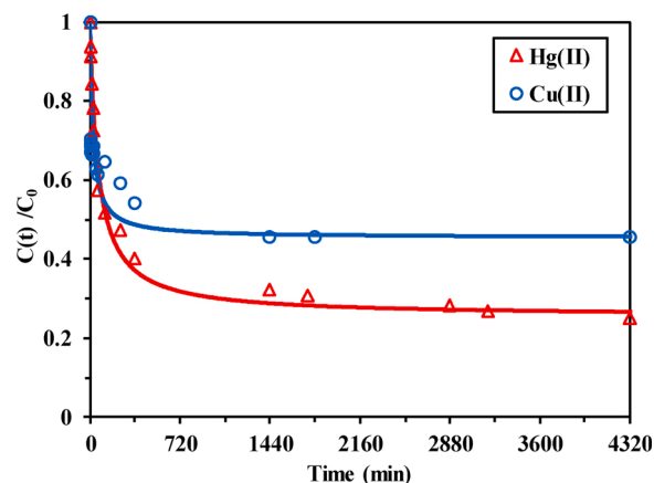
Fig. 1. Modeling of kinetic profiles (Metal concentration: 0.25 mmol L -1 of Cu (II) or Hg(II) single solution; Sorbent dosage = 0.2 g L -1 ; initial pH = 5; T: 20 ± 1 °C; solid line: fit of kinetic profile with the PSORE).
