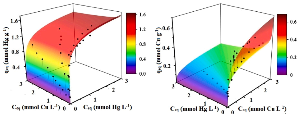
Fig. 3. Three-dimensional sorption surface plot showing competitive Sips model prediction and experimental data points.
