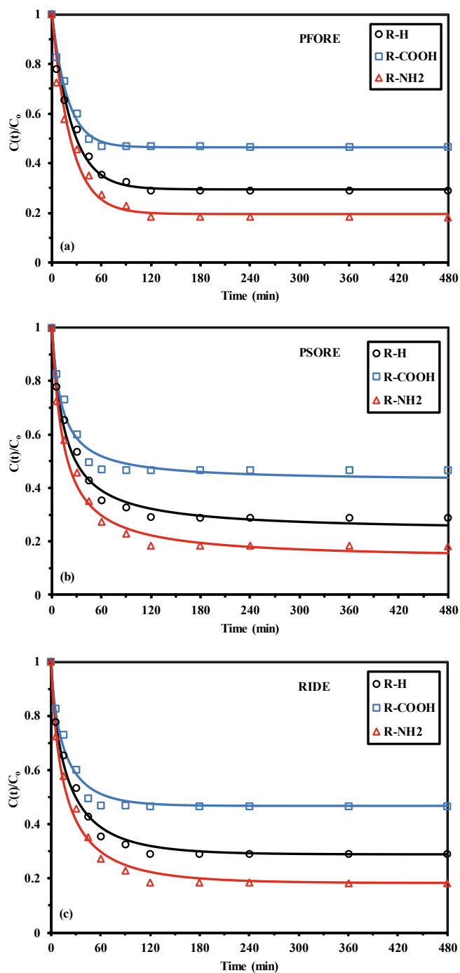
Fig. 4. Uptake kinetics for U(VI) sorption using R-H, R-COOH, and R-NH 2 sorbents – Modeling with PFORE, PSORE and RIDE ( pH_0 : 4.02; C_0 : 0.325 mmol U\ L^{-1} ; T : 25 °C; SD : 0.5 g\ L^{-1} ; agitation speed: 200 rpm).
