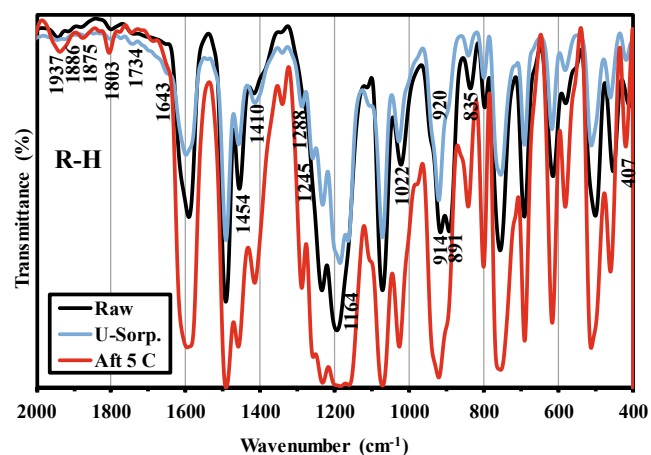
Fig. 2a. FTIR spectra of R-H before (raw) and after U(VI) sorption (U-Sorp.) and after 5 cycles of sorption and desorption (Aft.5C).
