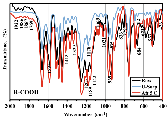
Fig. 2b. FTIR spectra of R-COOH before (raw) and after U(VI) sorption (U-Sorp.) and after 5 cycles of sorption and desorption (Aft.5C).
