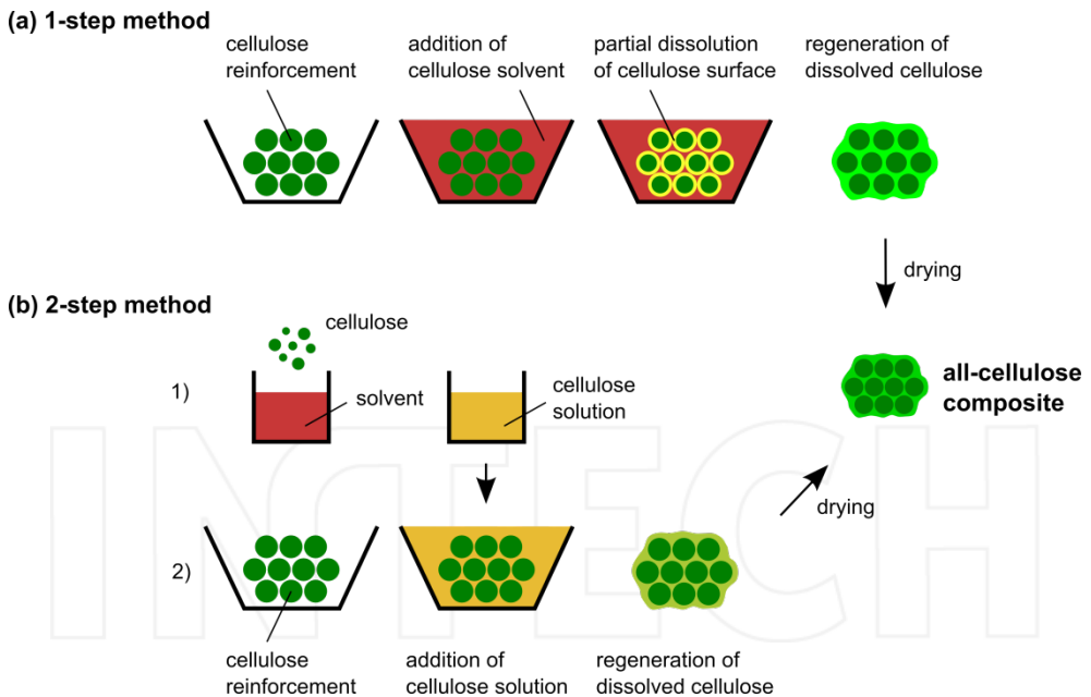
Figure 5. Schematic of processing pathways of ACCs: (a) One-step method and (b) Two-step method. Adapted from Nishino et al. [177].
