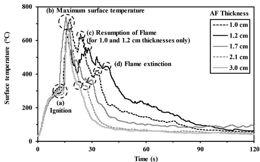
Fig. 6. Surface temperature of Alginite Foam with different thicknesses at 50 \text{ kW m}^{-2} heat flow.
