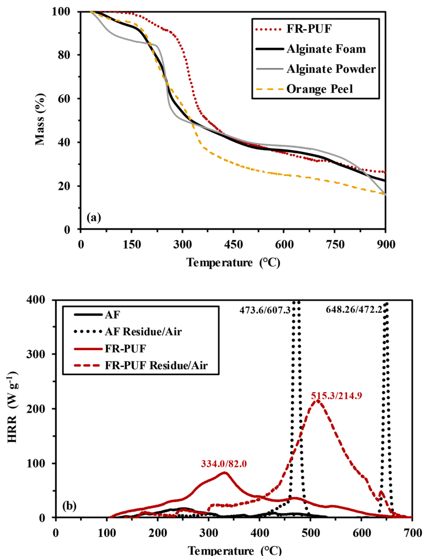
Fig. 3. Fire properties at microscale for AF and FR-PUF – (a) TGA curves, and (b) PCFC, HRR vs. Temperature for Alginate Foam (AF) and PUF (Anaerobic pyrolysis and aerobic pyrolysis of residues).
