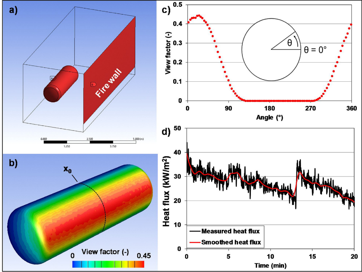
Fig. 2 – Boundary condition definition process: 3D geometry for view factors calculation (a), contour plot of the view factor (b), view factors on the section x_0 as a function of the angle \theta (see Fig. 1) (c), measured and smoothed heat flux obtained by the flux meter (d). The boundary conditions are implemented in FLUENT through the UDF reported in Appendix A.3.
