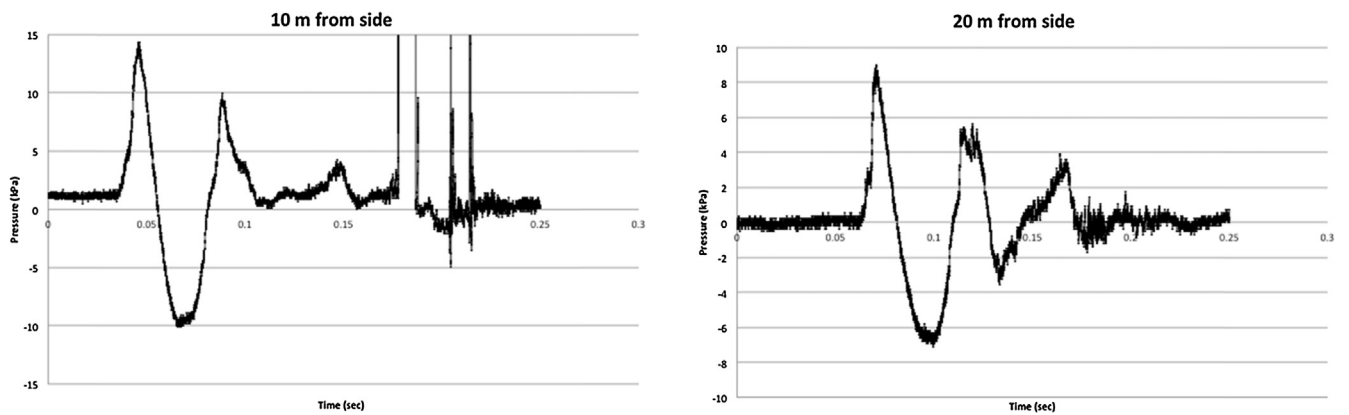
Fig. 3 – Overpressure measured at 10 m (left) and 20 m (right) from side of 1.9 m 3 propane tank.
