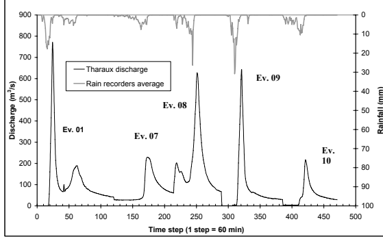
Fig. 2: Floods Hydrographs of the Cèze (Tharaulx outlet)
