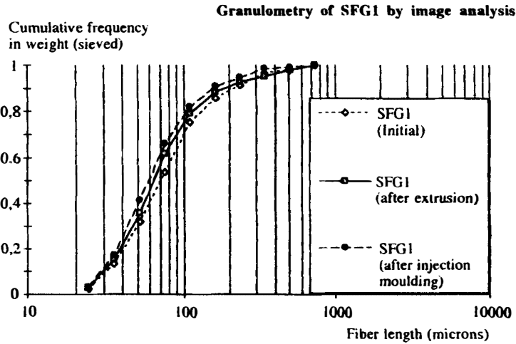
FIGURE 3 Evolution of SFG1 granulometry (in weight) with the processing.
