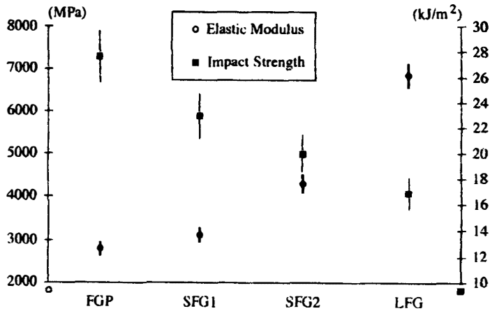
FIGURE 5 Results of impact and tensile test on powder, short and long fibreglass.
