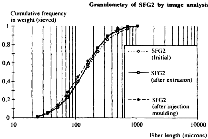
FIGURE 4 Evolution of SFG2 granulometry (in weight) with the processing.
