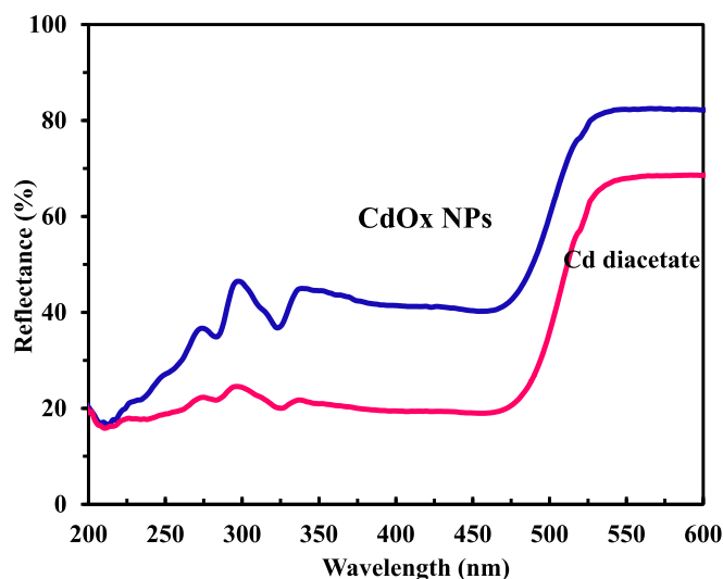
Fig. 1. Diffuse reflectance spectroscopy - UV-visible absorption spectra of CdOx NPs and Cd diacetate.
