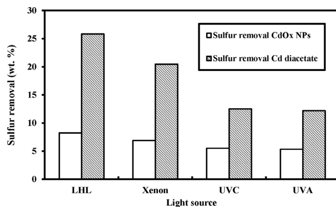
Fig. 5. Effect of the light source on sulfur removal (%) using CdOx NPs and Cd diacetate photocatalysts ([sulfur]: 11500 ppm; for liquid photocatalyst: identical volume of diesel and molar \text{Cd}(\text{CH}_3\text{COO})_2 solution; for Cd NPs: the solid/liquid ratio was set to 7 \text{ g L}^{-1} ; reaction time: 3 h at room temperature, using different irradiation systems; agitation speed: 500 rpm; separation: 45-min settling time or filtration, respectively) Note: these data are representing the effective effect of light irradiation (the specific adsorption effect of the catalytic phase is not taken into account in the removal efficiency).
