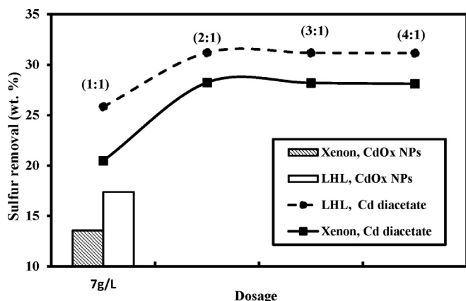
Fig. 6. Effect of (\text{Cd}(\text{CH}_3\text{COO})_2 and CdOx NPs)/diesel feed stock on sulfur removal ([sulfur]: 11500 ppm; for liquid photocatalyst: variable volume ratio of molar \text{Cd}(\text{CH}_3\text{COO})_2 solution/diesel (1:1 to 4:1); for Cd NPs: the solid/liquid ratio was set to 7 \text{ g L}^{-1} ; reaction time: 3 h at room temperature, under visible irradiation: Xenon or LHL lamp; agitation speed: 500 rpm; separation: 45-min settling time or filtration) Note: here the sulfur removal efficiency takes into account the contributions of both photocatalytic activity and adsorption.
