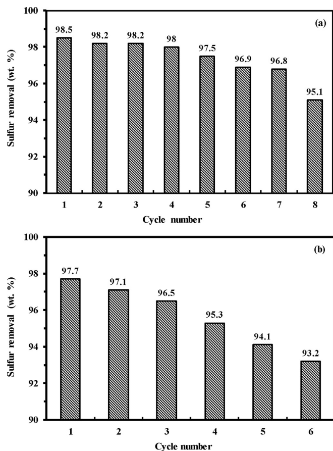
Fig. 10. Effect of catalyst recycling on desulfurization efficiency: (a) Cd diacetate, (b) CdOx NPs (Reaction Conditions: light: LHL; reaction time: 2 h; room temperature; \text{Cd}(\text{CH}_3\text{COO})_2/\text{Feed}/\text{H}_2\text{O}_2 ; 2:1:1 and S/F = 2:1; for CdOx NPs: catalyst dosage: 7 g L -1 ; Feed/ \text{H}_2\text{O}_2 /AcOH = 1:1:1; and S/F = 4/1).
