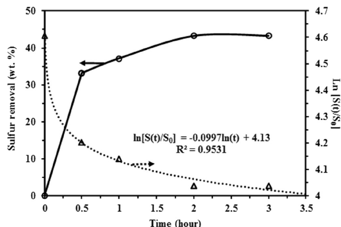
Fig. 8. Effect of reaction time on sulfur removal (%) using Cd diacetate photocatalyst (Cd diacetate/Feed/ H_2O_2 (30%) = 2:1:1; conditions; room temperature; settling time: 45 min; under LHL irradiation).
