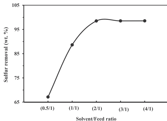
Fig. 9. Effect of solvent/feed ratio on sulfur removal (Cd diacetate/Feed/ H_2O_2 (30%) = 2:1:1; room temperature; stirring speed: 500 rpm; settling time: 45 min; under LHL irradiation; separation at room temperature with Solvent/feed ratio: 0.5:1 to 4:1).
