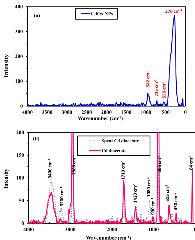
Fig. 4. Raman spectra of a) as-prepared CdOx NPs and b) freshly synthesized Cd diacetate photocatalysts and spent photocatalyst.
