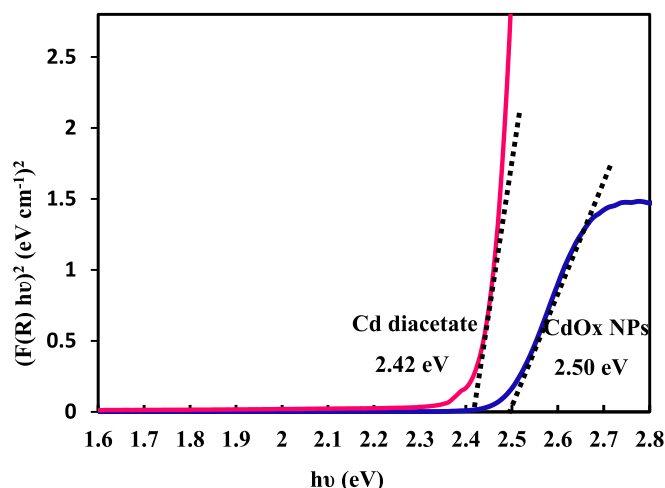
Fig. 2. Optical band gap energies for CdOx NPs and Cd diacetate photocatalysts.
