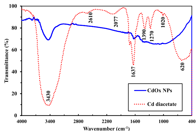
Fig. 3. IR spectra of as-prepared CdOx NPs and freshly synthesized Cd diacetate liquid.
