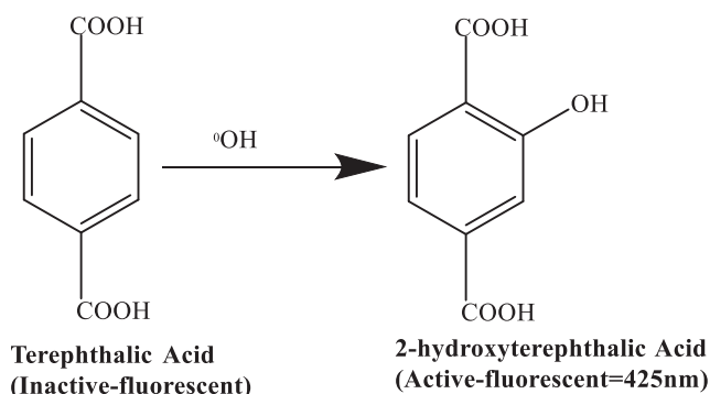
Scheme 1. The reaction of terephthalic acid with the hydroxyl radicals.
