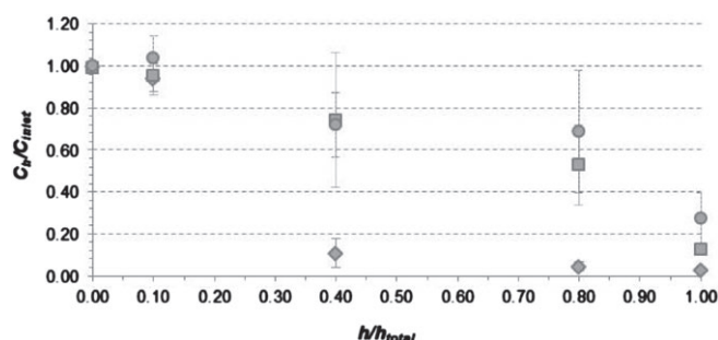
Figure 4. Concentration profiles of sulphur compounds along biofilter height. Hydrogen sulphide \diamond , methylmercaptan \blacksquare , dimethyldisulphide \bullet . The concentration ratio C_h/C_{inlet} was plotted against the height ratio h/h_{total} , where C_h is the outlet concentration ( \text{mg m}^{-3} ) at the height h of the biofilter (m), C_{inlet} the inlet concentration ( \text{mg m}^{-3} ) and h_{total} the total height of the column (2 m). For each compound, the results obtained for different gas samples were averaged.
