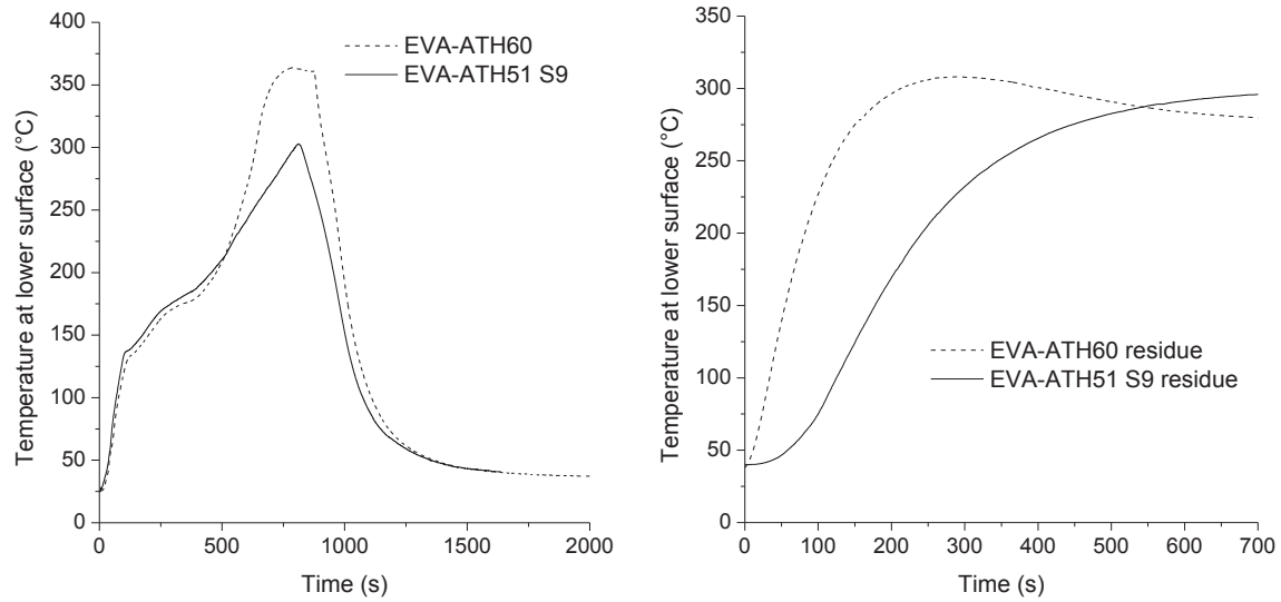
Fig. 5. Temperature of the lower surface during instrumented epi-radiator test – Left, for ATH60 and ATH51 S9 formulations; right, for corresponding residues.
