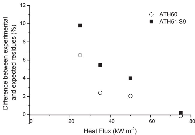
Fig. 4. Difference between measured and calculated residues for ATH60 and ATH51 S9 for various heat fluxes.
