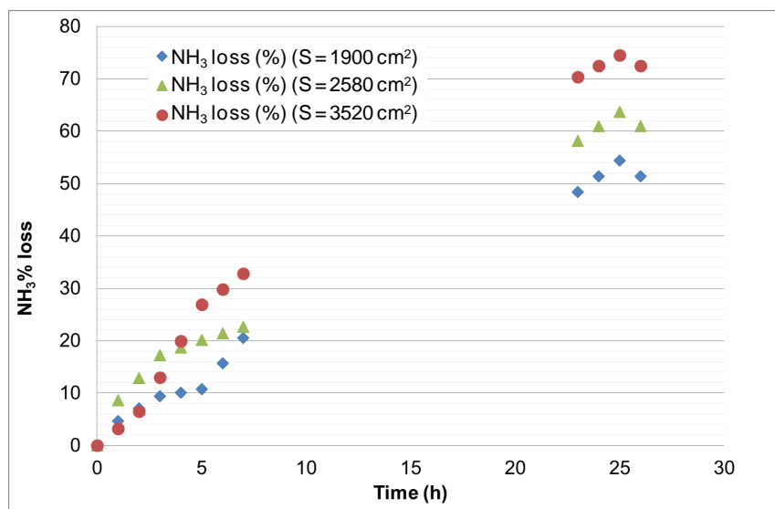
Figure 6. NH 3 loss (%) over time from the three bags having different surfaces (1900 cm 2 , 2580 cm 2 and 3520 cm 2 , respectively) and different S/V ratios (0.63 cm -1 , 0.86 cm -1 and 1.17 cm -1 , respectively).
