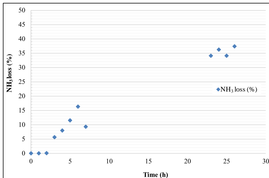
Figure 3. NH 3 loss (%) over time from the Nalophan™ bag with V_N = 6000 \text{ cm}^3 and S_N = 2580 \text{ cm}^2 .
