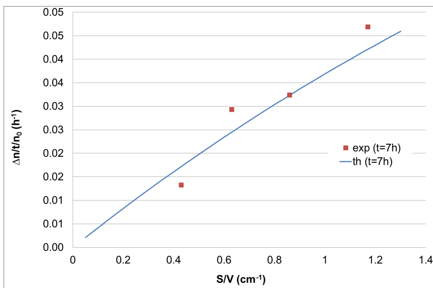
Figure 7. Average permeation speed (t = 7 h) normalized with respect to n_0 for different values of S/V.
