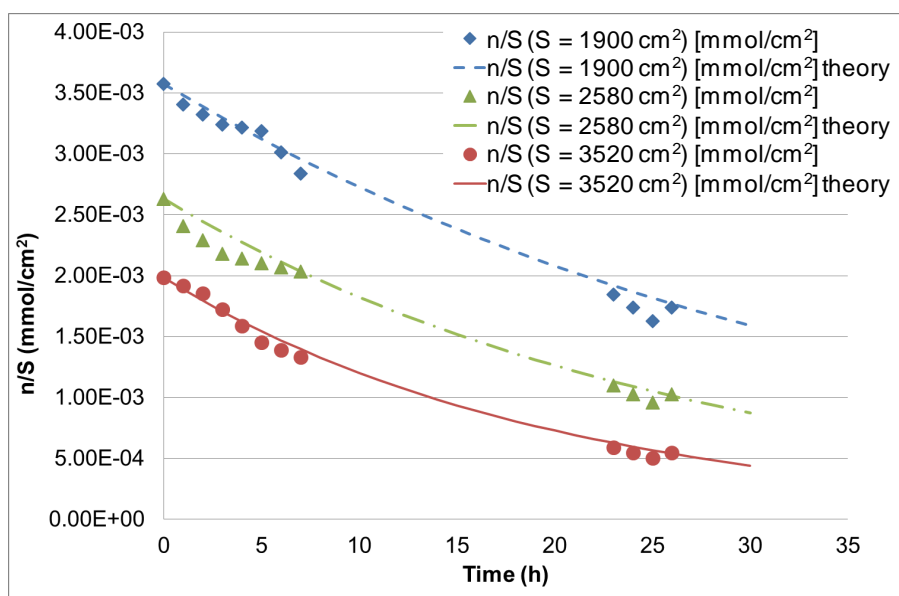
Figure 5. n/S trends for the three bags having different surfaces ( 1900 \text{ cm}^2 , 2580 \text{ cm}^2 and 3520 \text{ cm}^2 , respectively) and different S/V ratios ( 0.63 \text{ cm}^{-1} , 0.86 \text{ cm}^{-1} and 1.17 \text{ cm}^{-1} , respectively).
