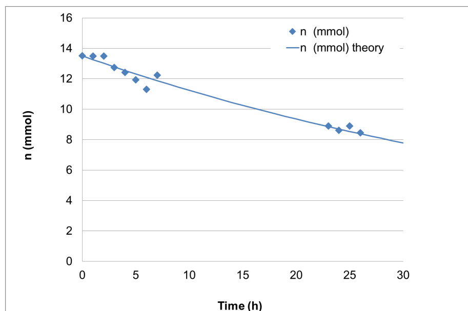
Figure 4. Number of NH 3 moles over time: experimental data (dots) vs. theoretical trend (continuous line) in a Nalophan™ bag with V_N = 6000 \text{ cm}^3 and S_N = 2580 \text{ cm}^2 .
