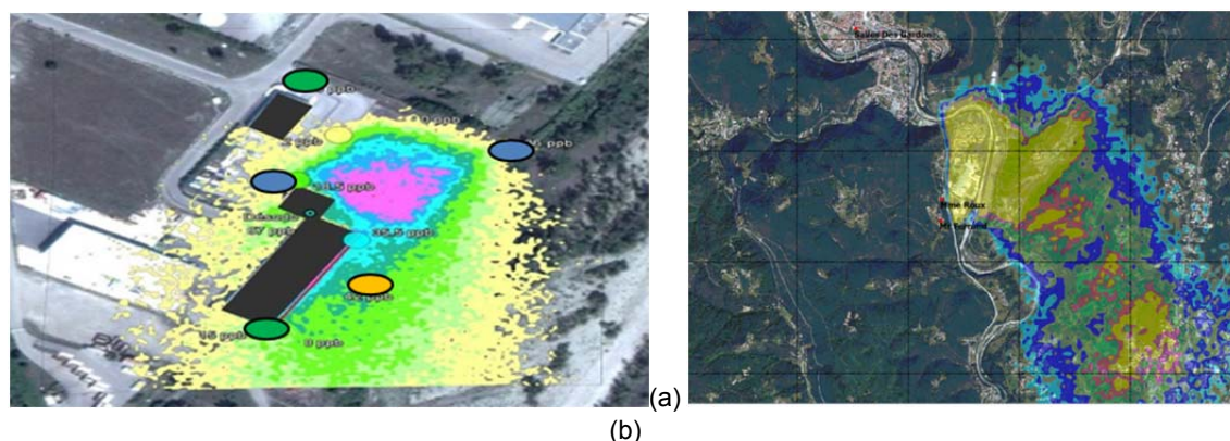
Figure 7: (a) Determination of emission sources by reverse modelling, (b) Dispersion model of \text{NH}_3
