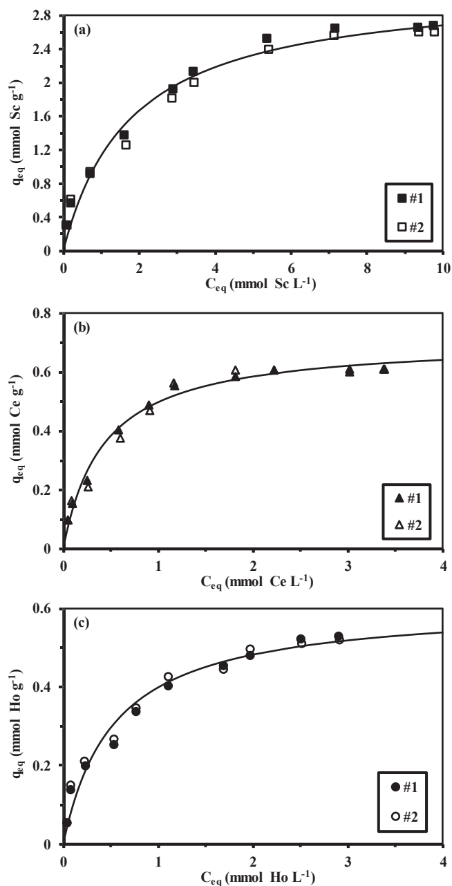
Fig. 5. Sorption isotherms for Sc(III) (a), Ce(III) (b) and Ho(III) (c) using S-A 1 PEI at pH 0 5 – modeling with the Langmuir equation (solid lines; duplicates, Langmuir data calculated from cumulative curves; SD: 0.5 g L -1 ; pH eq : 3.9–3.4; T: 22 ± 2 °C; contact time: 48 h; agitation speed: 170 rpm).
