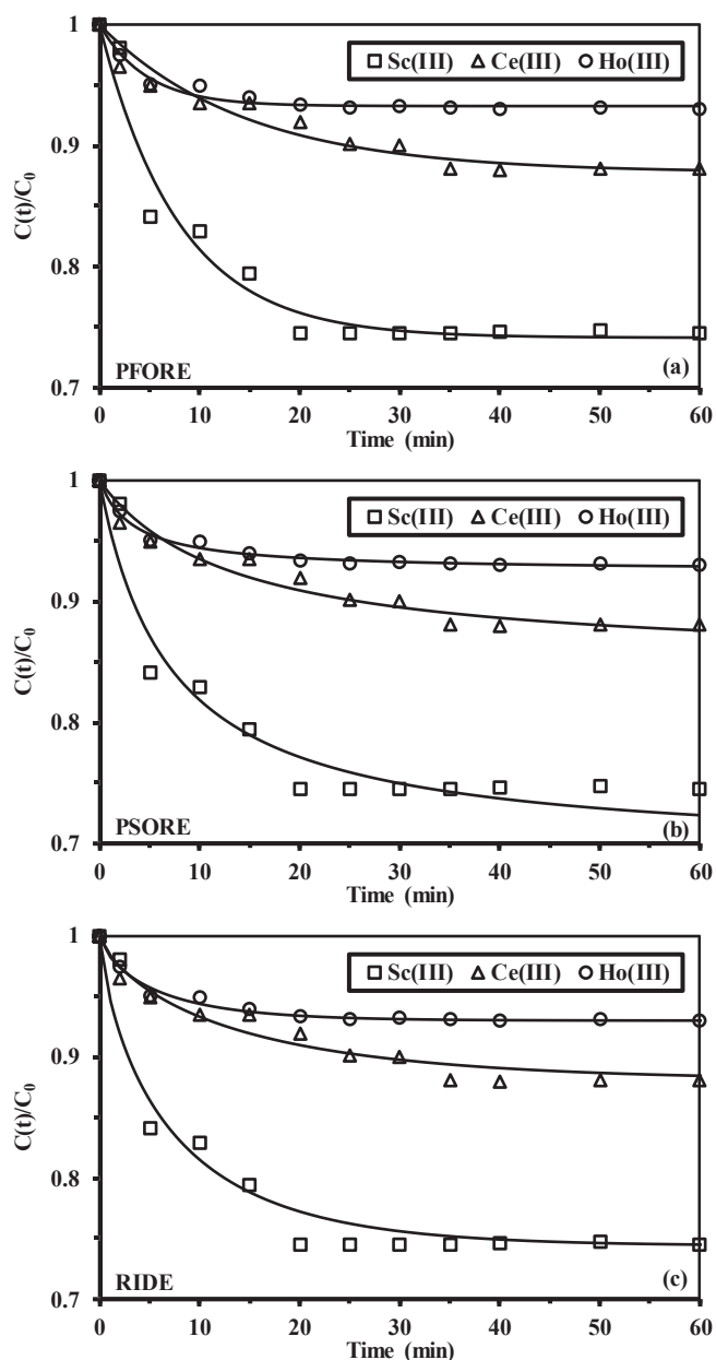
Fig. 4b. Uptake kinetics for multi-component solutions at pH 0 5 using S-A 1 PEI – Modeling with the PFORE, PSORE and RIDE ( C_0 : 0.25 mM; SD: 0.25 g L -1 ; pH eq : 3.6; T: 22 ± 2 °C; agitation speed: 170 rpm).
