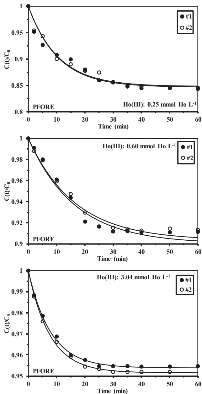
Fig. 3c. Ho(III) uptake kinetics at pH 0 5 using S-A 1 PEI – Modeling with the PFORE (C 0 : 0.60 mmol Ho L -1 and 3.04 mmol Ho L -1 ; SD: 0.25 g L -1 ; pH eq : 3.9–3.7; T: 22 ± 2 °C; agitation speed: 170 rpm).
