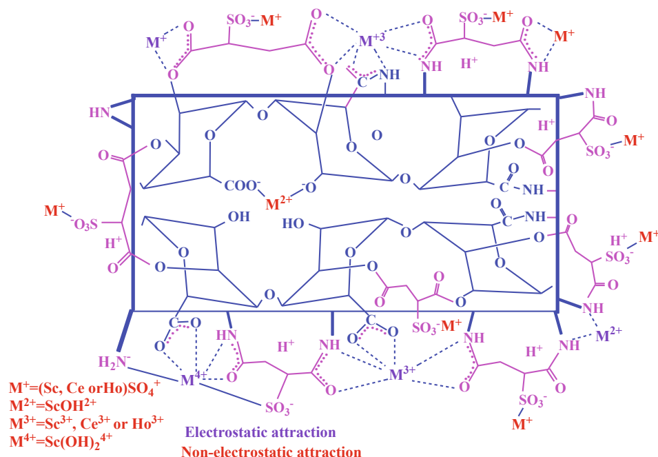
Scheme 2. Suggested mechanisms of interaction between S-A 1 PEI and REEs metal ions.
