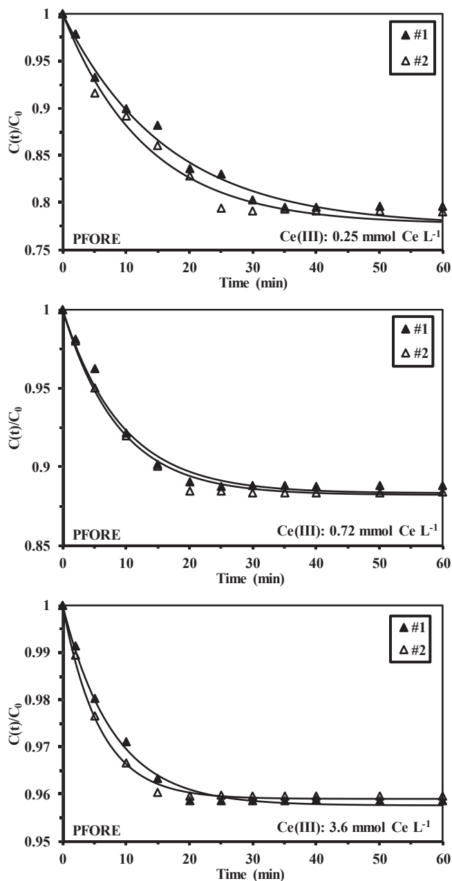
Fig. 3b. Ce(III) uptake kinetics at pH 0 5 using S-A 1 PEI – Modeling with the PFORE (C 0 : 0.25, 0.72 and 3.6 mmol Ce L -1 ; SD: 0.25 g L -1 ; pH eq : 3.7–3.4; T: 22 ± 2 °C; agitation speed: 170 rpm).
