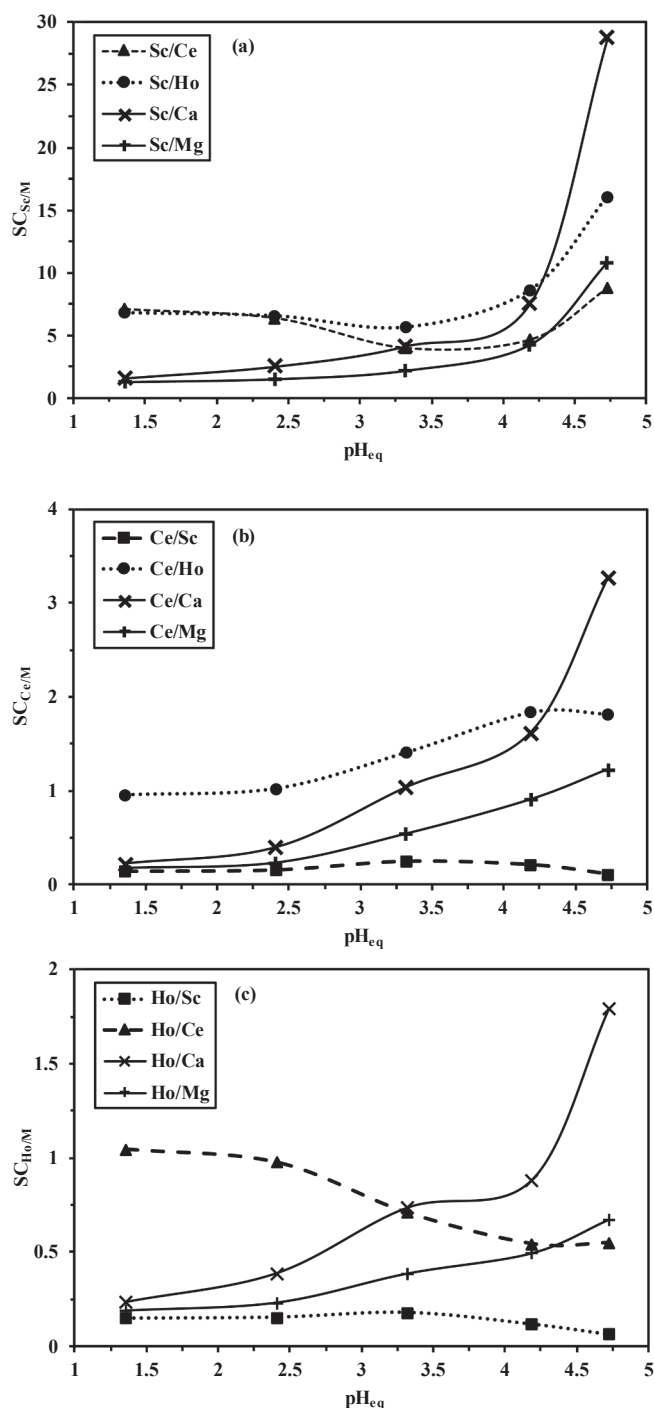
Fig. 6. Selectivity coefficients for Sc(III) (a), Ce(III), and Ho(III) sorption against other metal ions (REEs and alkali-earth Ca(II) and Mg(II) metal ions) as a function of equilibrium pH (equimolar metal concentrations: 1 mmol L -1 ; SD: 2 g L -1 ; T: 22 ± 2 °C; contact time: 48 h; agitation speed: 170 rpm).
