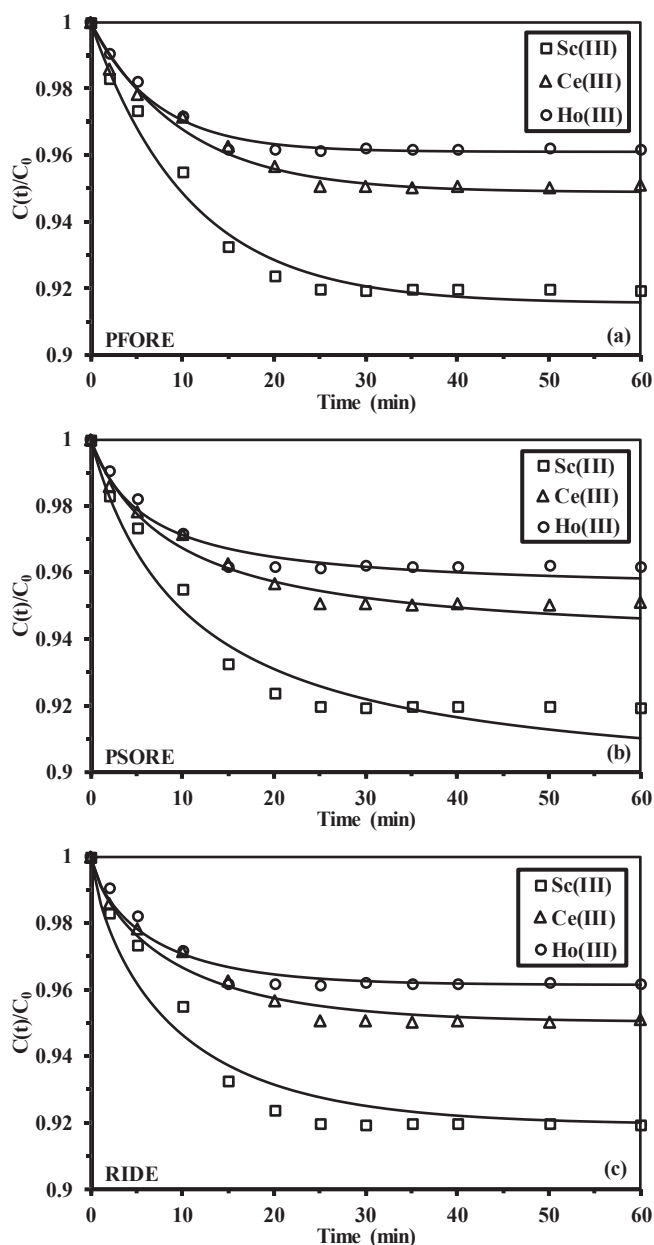
Fig. 4a. Uptake kinetics for multi-component solutions at pH 0 5 using S-A 1 PEI – Modeling with the PFORE, PSORE and RIDE ( C_0 : 100 mg L -1 ; SD: 0.25 g L -1 ; pH eq : 3.6; T: 22 ± 2 °C; agitation speed: 170 rpm).
