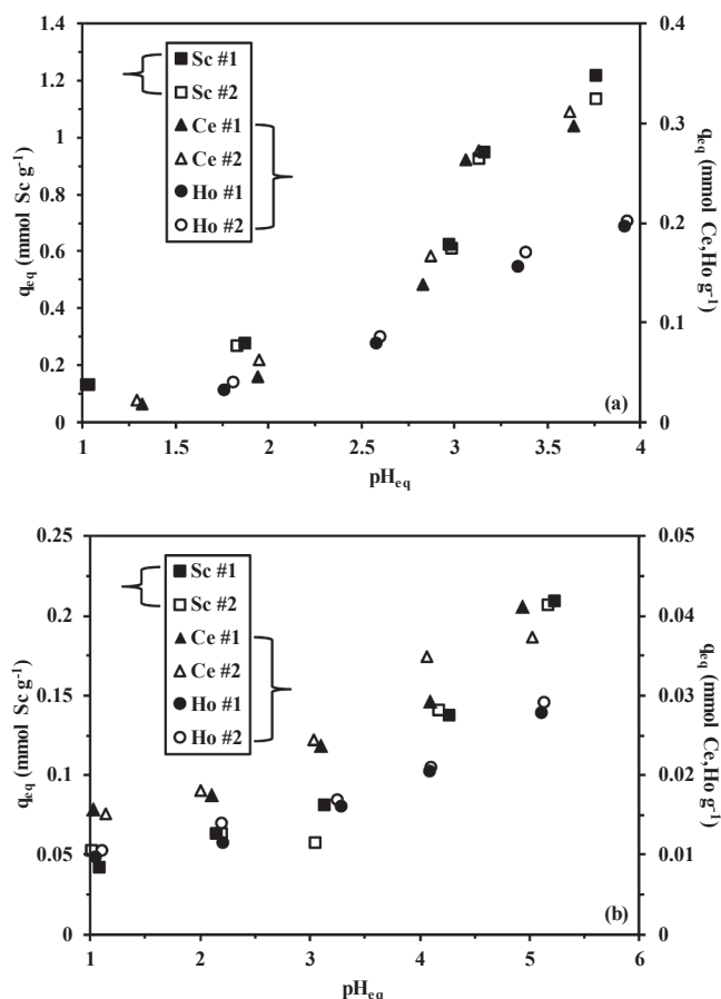
Fig. 2. Effect of pH on REE(III) sorption using S-A L PEI (a) and A L PEI (b) (C 0 : 100 mg L -1 ; or 2.3 mmol Sc L -1 , 0.72 mmol Ce L -1 , 0.65 mmol Ho L -1 ; Sorbent dosage, SD: 166 mg L -1 ; contact time: 48 h; T: 22 ± 2 °C; agitation speed: 170 rpm).
