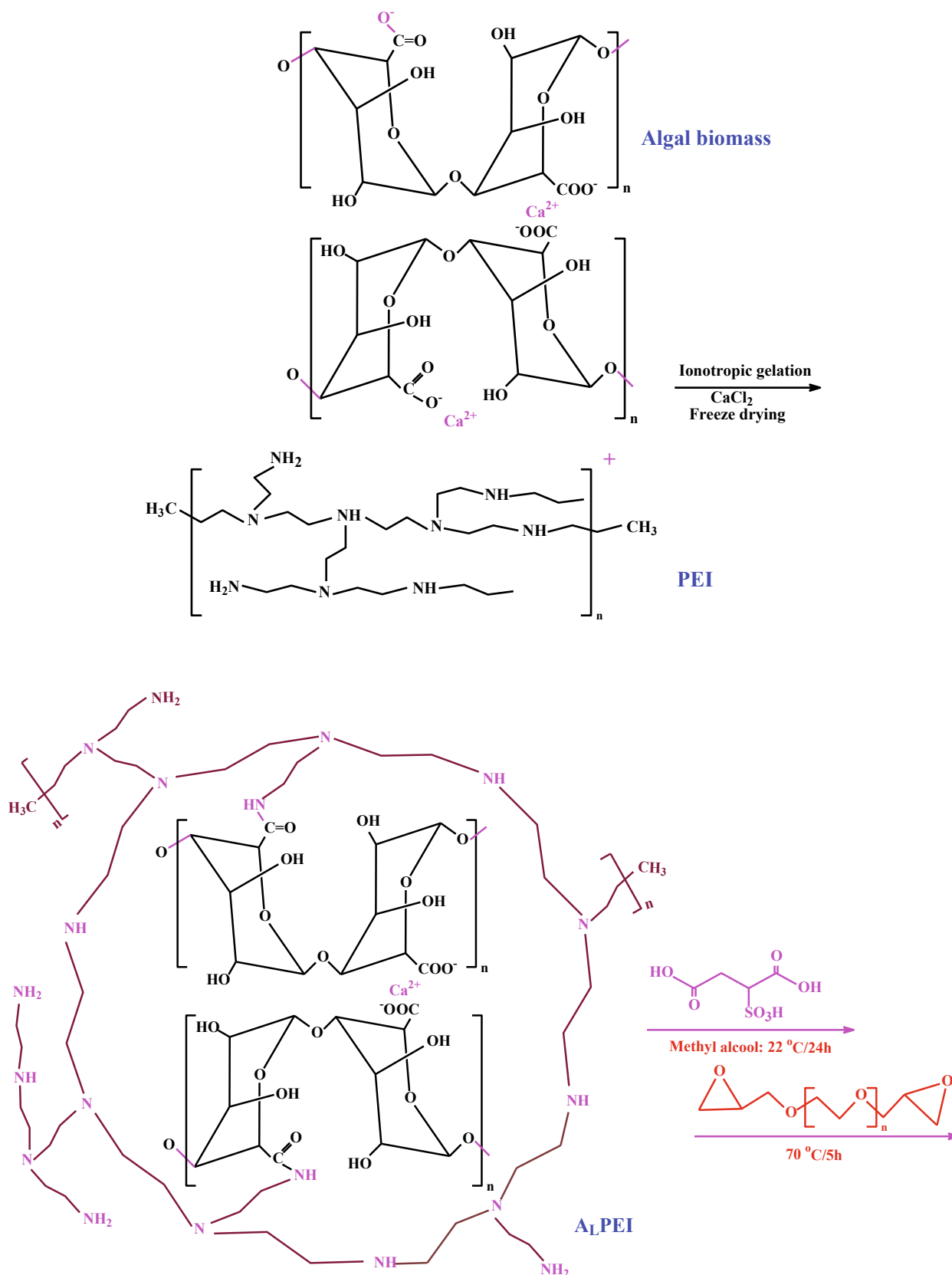
Scheme 1. Synthesis procedure – Expected (simplified) structure of the sorbent (algal biomass simplified to alginate active material).
