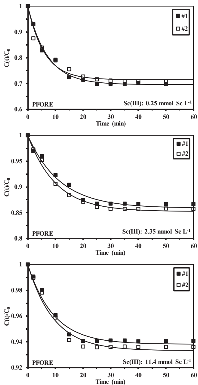
Fig. 3a. Sc(III) uptake kinetics at \text{pH}_0 5 using \text{S-A}_1\text{PEI} – Modeling with the PFORE ( C_0 : 0.25, 2.35 and 11.4 mmol \text{Sc L}^{-1} ; \text{SD} : 0.25 \text{g L}^{-1} ; \text{pH}_{\text{eq}} : 3.8–3.4; T : 22 \pm 2 °C; agitation speed: 170 rpm).
