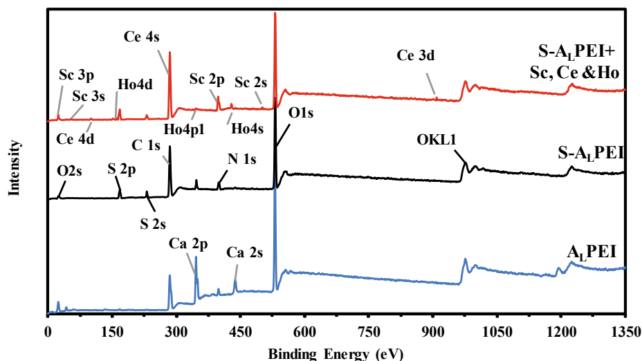
Fig. 1. XPS survey spectra of A L PEI, S-A L PEI, and S-A L PEI after binding of Sc(III), Ce(III) and Ho(III) (multi-component solution).
