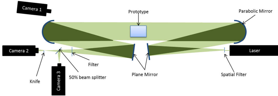
Fig. 3 Optical setup
