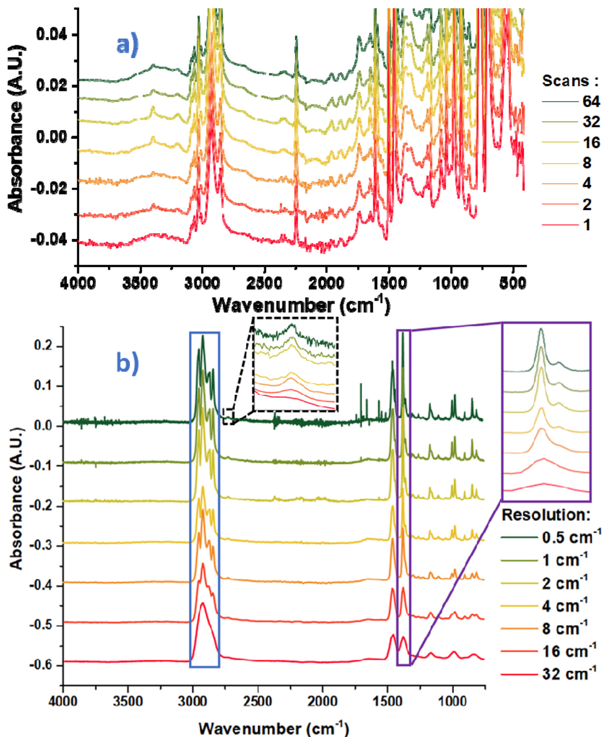
Figure 2. Impacts of acquisition parameters in FTIR-ATR on the quality of spectra: a) Number of scans reduction on an ABS standard with a 4 cm -1 resolution b) Resolution degradation on a PP standard with 1 scan per measure – blue frame for C-H stretching convoluting signals and purple for crystallinity marker
