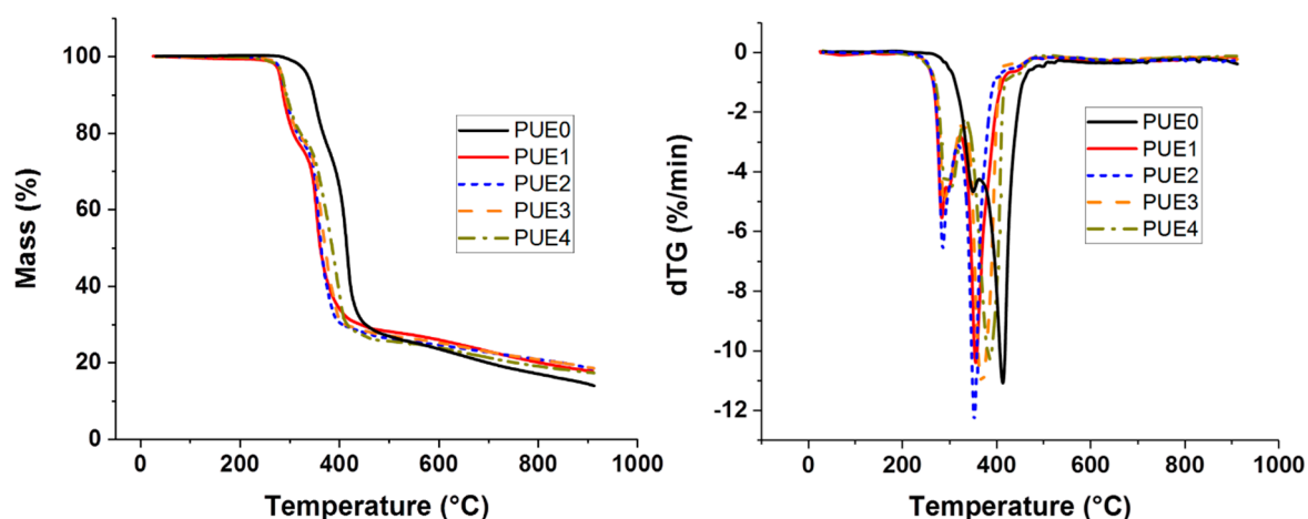
Figure 7. TG and derivates of thermogravimetric curve (DTG) for PUE/APP/S9 composites.
