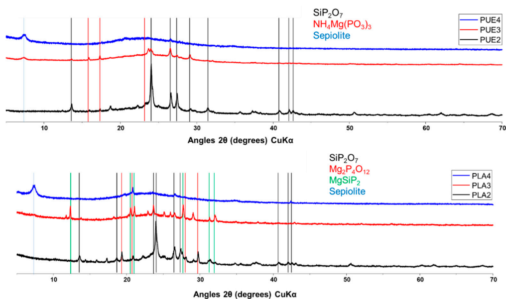
Figure 18. XRD patterns for PLA/APP/S9 and PUE/APP/S9 composites residues. (The colors of the vertical lines are in agreement with those of the compounds identified.)
