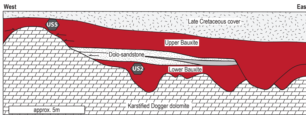
Fig. 5 : Cross section of the Bédarieux outcrop, showing the bauxite deposits (red) filling karstified dolomite and the location of samples US2 and US5. Two bauxite levels, separated by dolo-sandstones and marls, are onlapping the karst topography, and are covered by late Cretaceous conglomerates and sandstones. Note that the upper bauxite deposits are locally incised into the lower bauxite.
