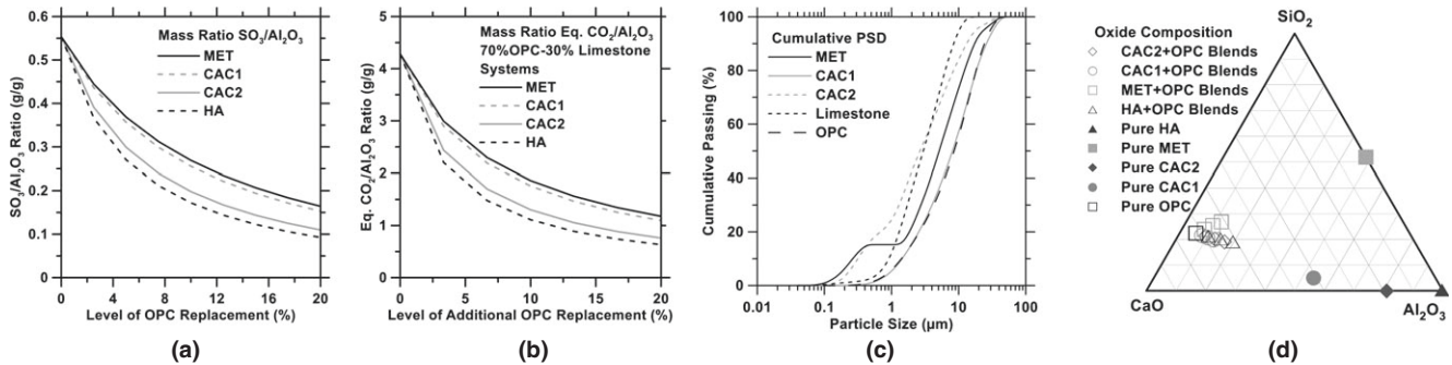
Fig. 1. (a) Sulfate-to-alumina ( \text{SO}_3/\text{Al}_2\text{O}_3 ) mass ratio as a function of increasing OPC replacement by a given alumina source, (b) Carbon dioxide equivalent-to-alumina ( \text{CO}_2/\text{Al}_2\text{O}_3 ) mass ratio for the mixtures containing 30% of limestone (dosed by OPC replacement) as a function of increasing OPC replacement by a given alumina source, (c) The cumulative particle size distributions of the powders, and, (d) The compositions of the binders, minus limestone, plotted on a ternary composition diagram (with \text{CaO-SiO}_2\text{-Al}_2\text{O}_3 at the vertices).
